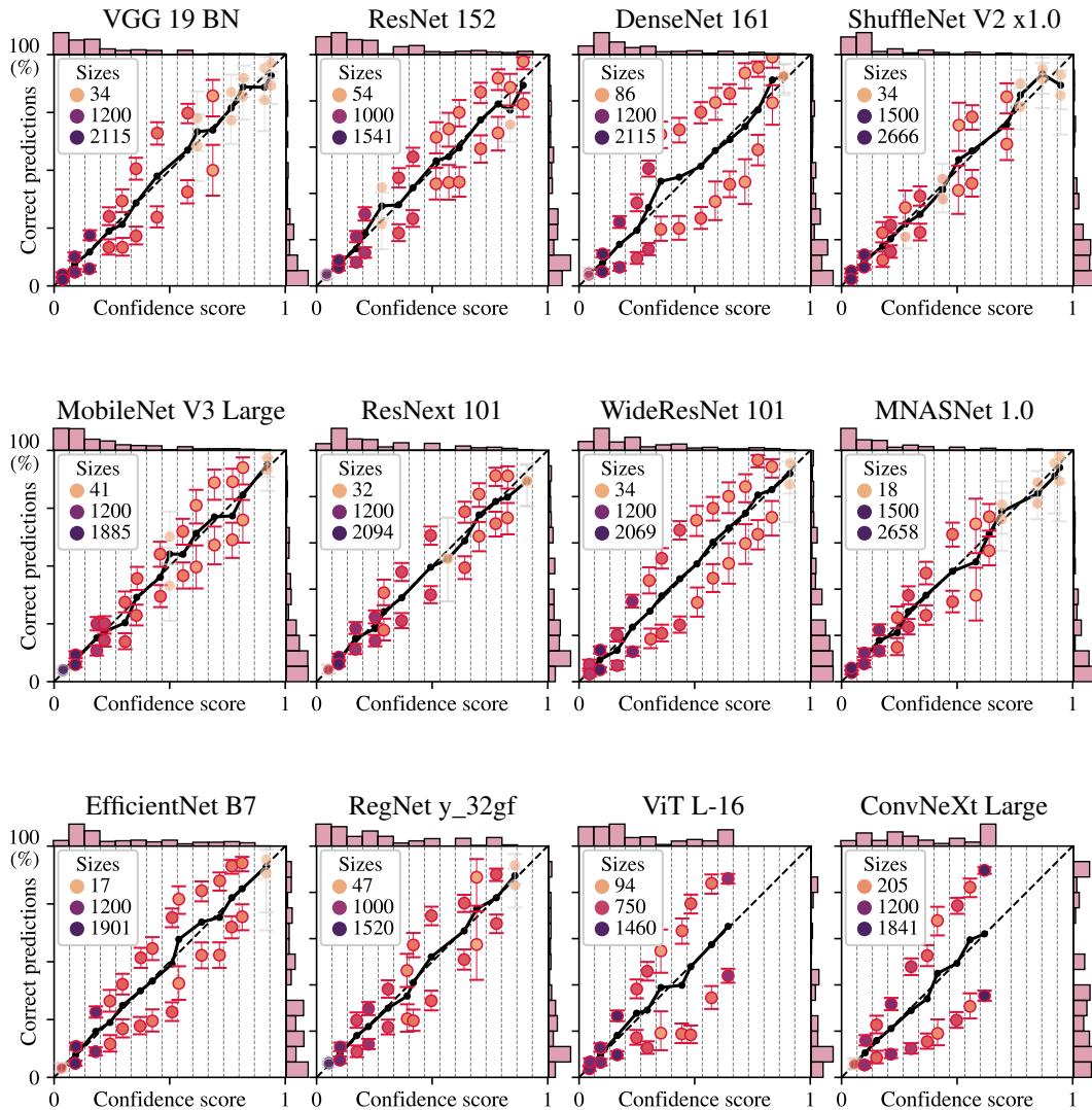
Figure 19: Vision : Fraction of correct predictions versus confidence score of predicted class ( \max_k S_k ) on ImageNet-R for best versions of pre-trained networks, with isotonic recalibration. In each bin on confidence scores, the level set is partitioned into 2 regions with a decision stump constrained to one balanced split, with a 50-50 train-test split strategy.
