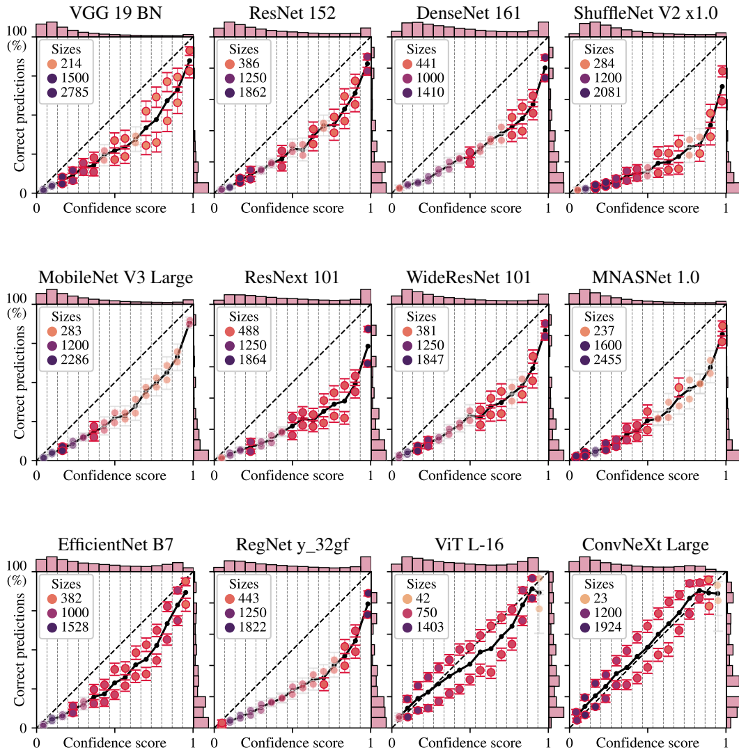
Figure 21: Vision : Fraction of correct predictions versus confidence score of predicted class ( \max_k S_k ) on ImageNet-C for best versions of pre-trained networks, without post-hoc recalibration. In each bin on confidence scores, the level set is partitioned into 2 regions with a decision stump constrained to one balanced split, with a 50-50 train-test split strategy.
