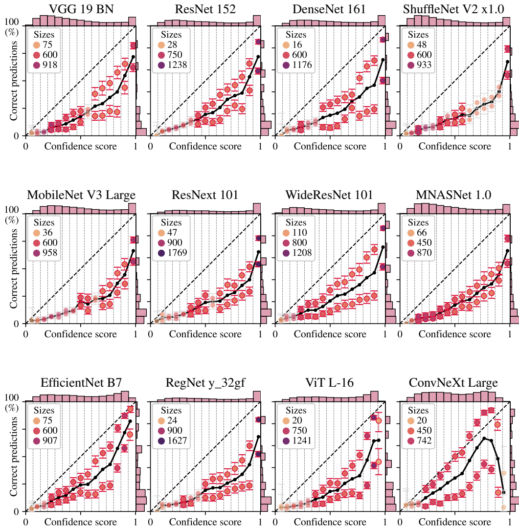
Figure 17: Vision : Fraction of correct predictions versus confidence score of predicted class ( \max_k S_k ) on Image NET -R for best versions of pre-trained networks, without post-hoc recalibration. In each bin on confidence scores, the level set is partitioned into 2 regions with a decision stump constrained to one balanced split, with a 50-50 train-test split strategy.
