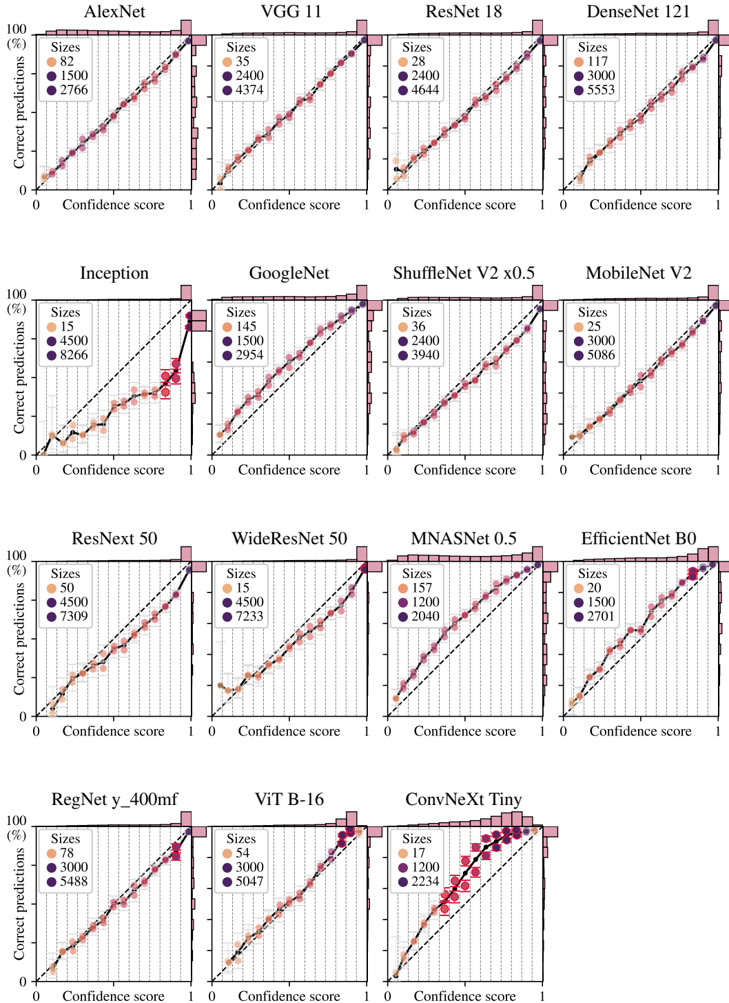
Figure 24: Vision : Fraction of correct predictions versus confidence score of predicted class ( \max_k S_k ) on ImageNet-1K (validation set) for small versions of pre-trained networks, without post-hoc recalibration. In each bin on confidence scores, the level set is partitioned into 2 regions with a decision stump constrained to one balanced split, with a 50-50 train-test split strategy.
