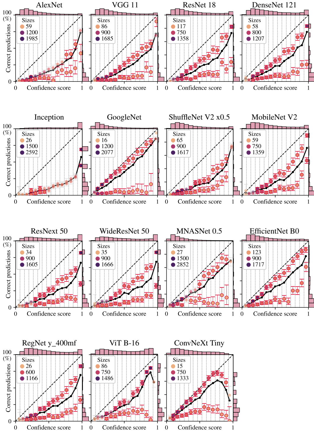
Figure 16: Vision : Fraction of correct predictions versus confidence score of predicted class ( \max_k S_k ) on ImageNet-R for small versions of pre-trained networks, without post-hoc recalibration. In each bin on confidence scores, the level set is partitioned into 2 regions with a k -means clustering, with a 50-50 train-test split strategy (for a fair comparison with decision stump clustering).
