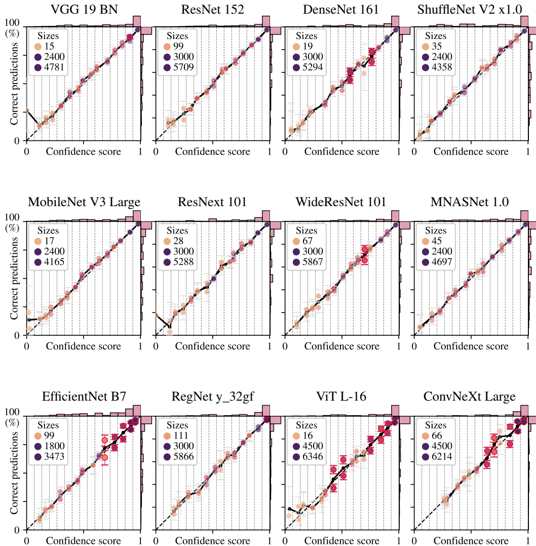
Figure 27: Vision : Fraction of correct predictions versus confidence score of predicted class ( \max_k S_k ) on ImageNet-1K (validation set) for best versions of pre-trained networks, with isotonic recalibration. In each bin on confidence scores, the level set is partitioned into 2 regions with a decision stump constrained to one balanced split, with a 50-50 train-test split strategy.
