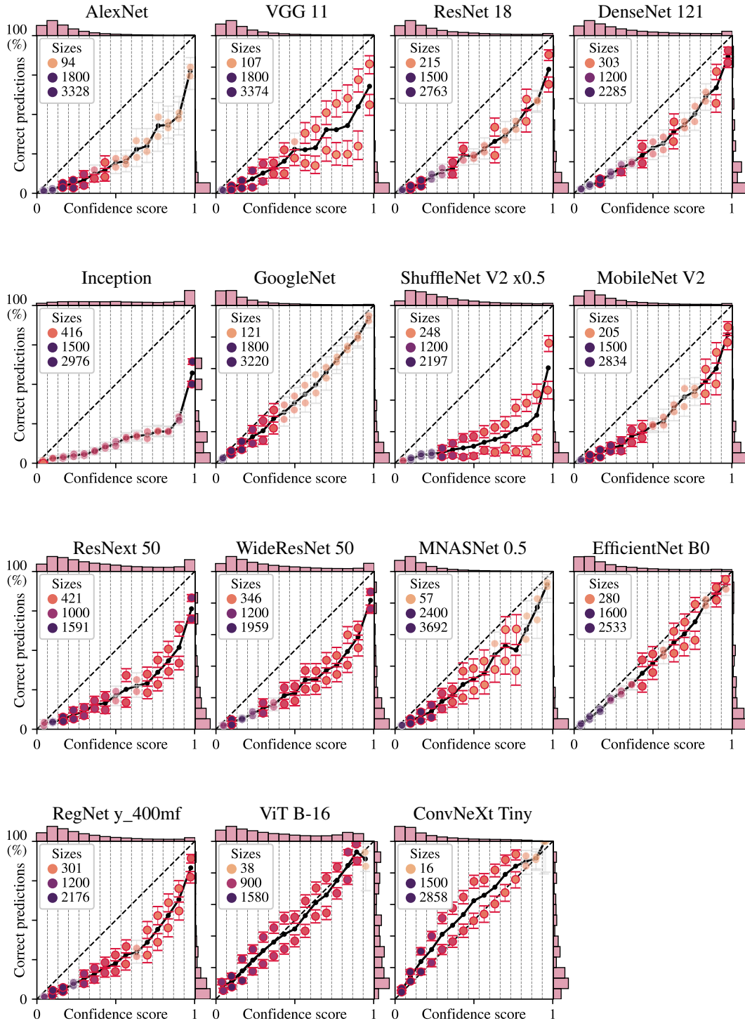
Figure 20: Vision: Fraction of correct predictions versus confidence score of predicted class ( \max_k S_k ) on ImageNet-C for small versions of pretrained networks, without post-hoc recalibration. In each bin on confidence scores, the level set is partitioned into 2 regions with a decision stump constrained to one balanced split, with a 50-50 train-test split strategy.
