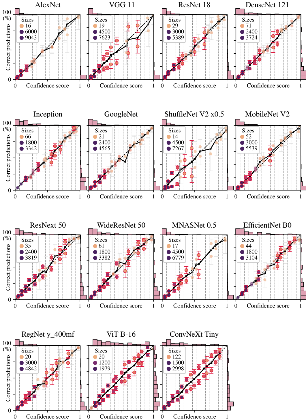
Figure 22: Vision : Fraction of correct predictions versus confidence score of predicted class ( \max_k S_k ) on ImageNet-C for small versions of pretrained networks, with isotonic calibration. In each bin on confidence scores, the level set is partitioned into 2 regions with a decision stump constrained to one balanced split, with a 50-50 train-test split strategy.
