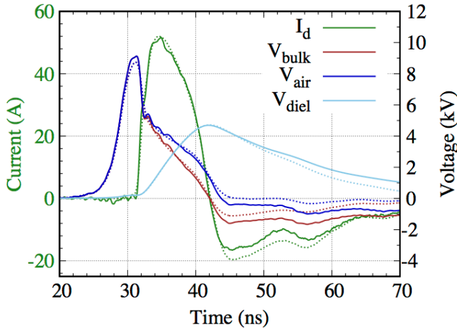
Fig. 7. Discharge current I_d (green). Voltage pulse applied to the air gap V_{air} (blue). Applied voltage to the plasma bulk V_{bulk} (red). Voltage applied to the dielectric layer V_{diel} (cyan). Experimental data are in solid lines and simulation results are in dotted lines.
