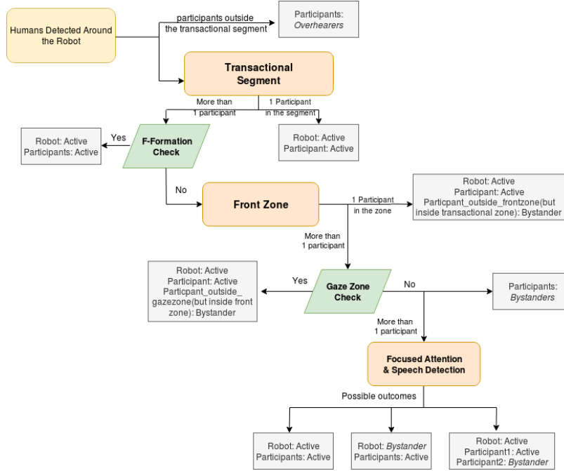
Fig. 3. Framework for Footing in Human-Robot Interaction
