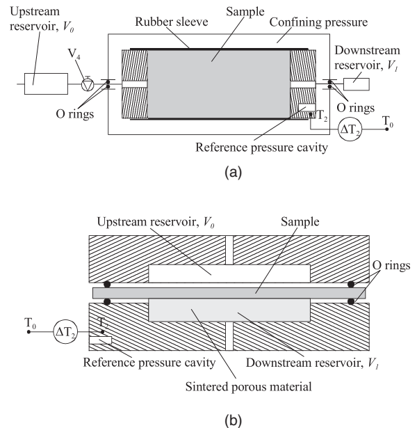
FIG. 6. Two measuring cells used for (a) a rock sample (Hassler sleeve core holder); (b) a composite material sheet.
