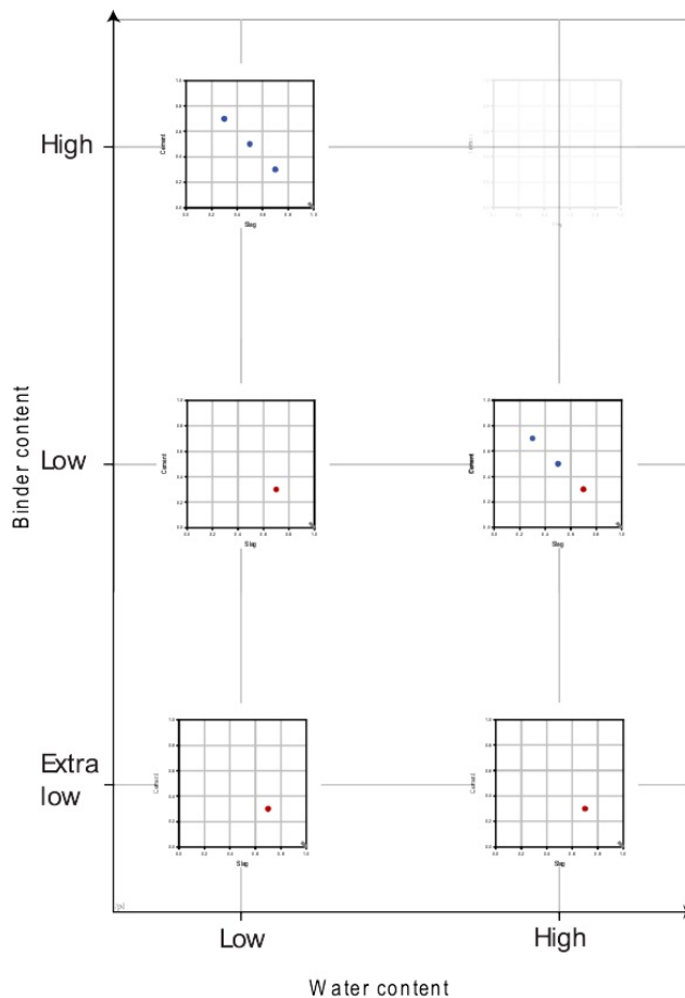
Fig. 5. Graph showing the setup of Phase 1 and 2 of the experiment. Here Phase 1 is indicated by the blue dots, Phase 2 – by the red dots. Blue circles show where Phases 1 and 2 overlap. High and low water ratios in these experiments consisted of 190%, respectively 139% (that is, excess of water).
