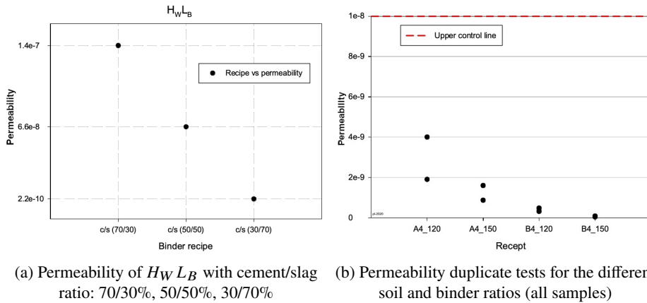
Fig. 7. Permeability tests on the stabilised soil with varied stabilising agents in different binder ratios
