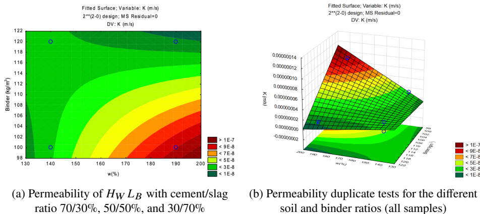
Fig. 8. Permeability tests on the stabilised soil with varied stabilising agents in different binder ratios
