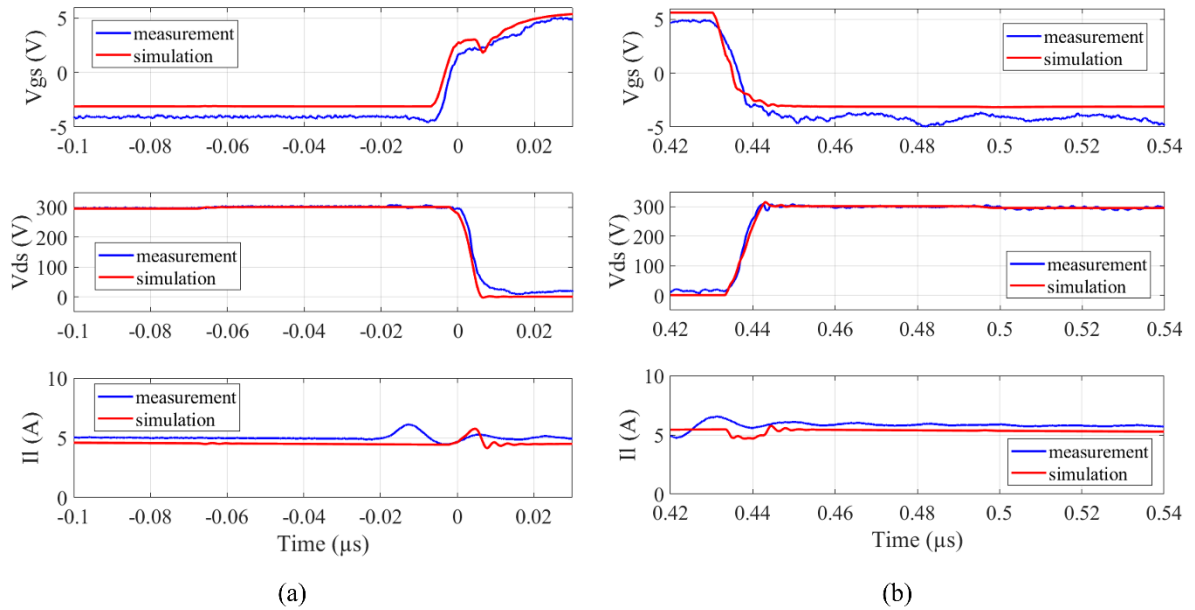
Fig. 9: Waveforms of the low-side GaN transistor and load current at (a) turn-on and (b) turn-off of the device
