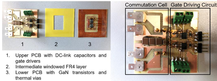
Fig. 3: Presentation of the fabricated parts and the assembly of the proposed M-PCB half-bridge
