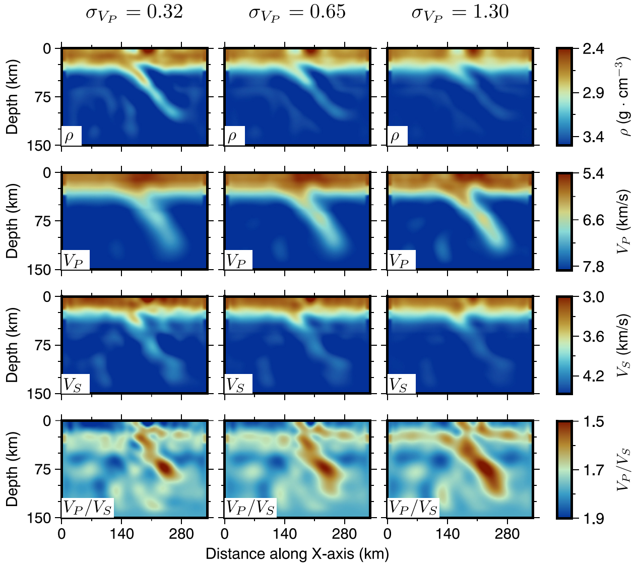
Figure 17. Comparison of long period FWI results for different \sigma_{V_P} ( \text{km s}^{-1} ). All the other hyperparameters are the same as in the reference inversion shown in Fig. 6.
