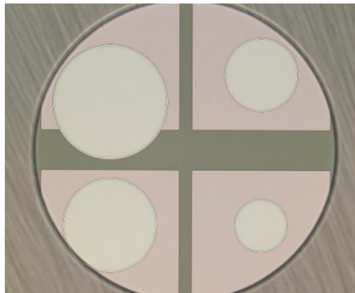
Figure 2: Frontside metal pads on GaN epitaxy seen from the backside through a trenced backside access cavity.
