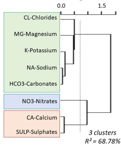
Fig. 4. Varclus and ClustOfVar dendrograms
