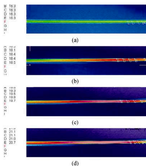
Figure 4. Surface temperature measured by Liu et al. [57] in a microtube of 44.2 \mu\text{m} inner diameter and 140 mm length at various Reynolds numbers. (a) Re=0 ; (b) Re=297.2 ; (c) Re=491.8 ; (d) Re=692 . Temperatures for various locations in the channel are provided in ^{\circ}\text{C} in the left part of
