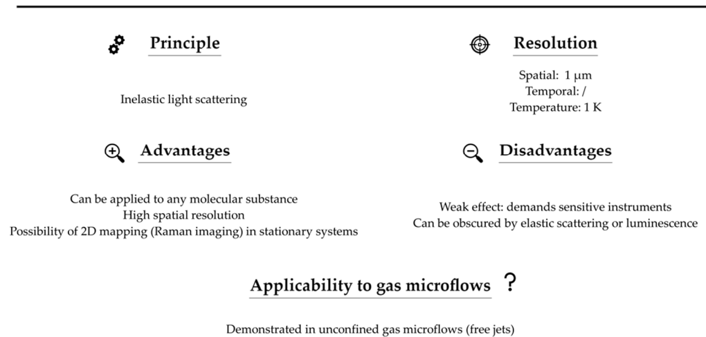
Figure 28. Summary of Raman thermometry features.
