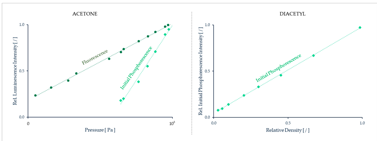
Figure 37. (a) (◆) Pressure dependence of acetone phosphorescence emission intensity collected for 100 \text{ ns} < t < 600 \text{ ns} , normalized by its value at atmospheric pressure for T = 294 \text{ K} and a molar fraction of acetone of 10.4%; (●) experimental fluorescence intensity collected for 0 < t < 10 \text{ ns} normalized by its value at atmospheric pressure. Data from Si Hadj Mohand et al. [184]. (b) Density dependence of initial phosphorescence intensity of diacetyl: the ordinate is normalized by the largest initial phosphorescence intensity of each experimental run, and the abscissa is normalized by the highest density of each experimental run. Data from Jian-Bang et al. [182].
