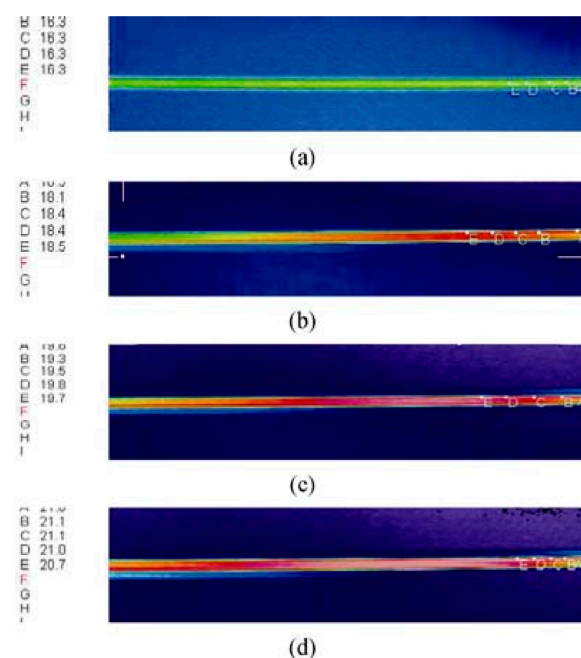
Figure 4. Surface temperature measured by Liu et al. [57] in a microtube of 44.2 \mu\text{m} inner diameter and 140 mm length at various Reynolds numbers. (a) Re=0 ; (b) Re=297.2 ; (c) Re=491.8 ; (d) Re=692 . Temperatures for various locations in the channel are provided in ^{\circ}\text{C} in the left part of
