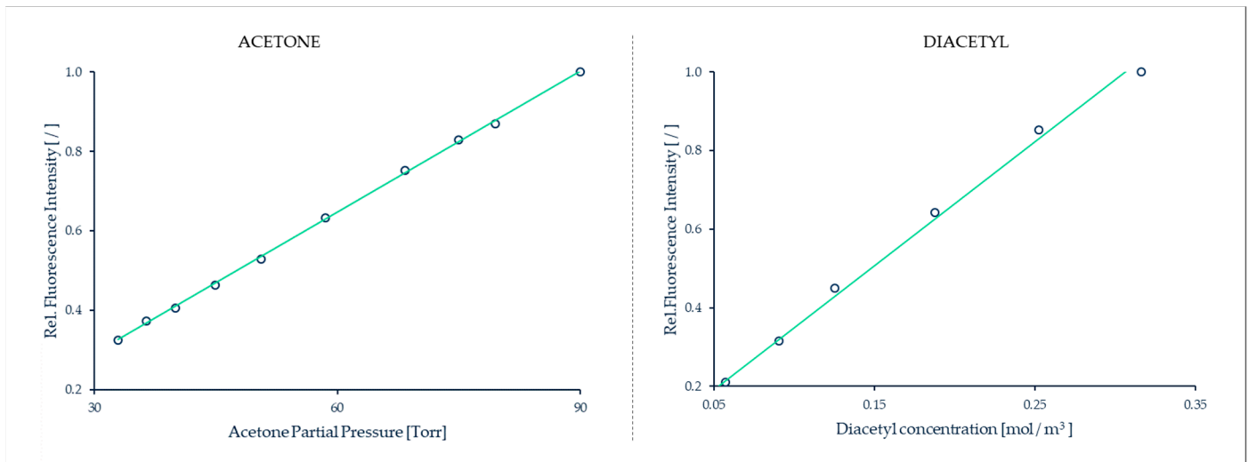
Figure 36. (a) Acetone fluorescence emission dependence on partial pressure, according to the data from Lozano et al. [171]; (b) Diacetyl fluorescence emission dependence on concentration (at constant temperature, this parameter is easily linked to pressure dependence), according to the data from Tomita et al. [183].
