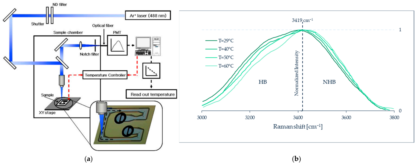
Figure 26. (a) Schematic diagram of the micro-Raman spectroscopy system used by Kim et al. Reprinted by permission from Ref. [142], Journal of Micromechanics and Microengineering, Copyright © 2022 IOP Publishing Ltd. (b) Changes in the OH stretching band of liquid water at different temperatures. Data from [142].
