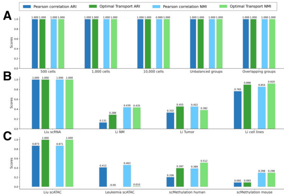
Fig. 3. Comparison of OT against Pearson correlation in hierarchical clustering. Barplots for ARI and NMI are reported for (A) simulated scRNA-seq data composed of 500, 1000 and 10000 cells, with unbalanced groups and overlapping clusters; (B) four scRNA-seq datasets; (C) two single-cell DNA methylation and two scATAC-seq data
