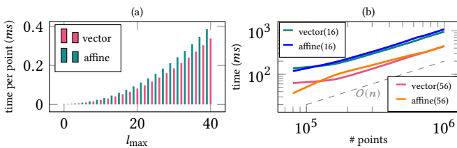
Fig. 13. Timing. For both vector and affine loads, we count: (a) per-point computational cost for a truncation of the SH series at l_{\max} ; (b) total computational cost with respect to the number of points evaluated for l_{\max} = 8 using 16 and 56 threads respectively.
