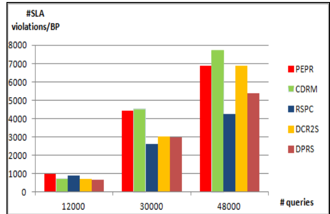
Figure 3 Average number of SLA violations
