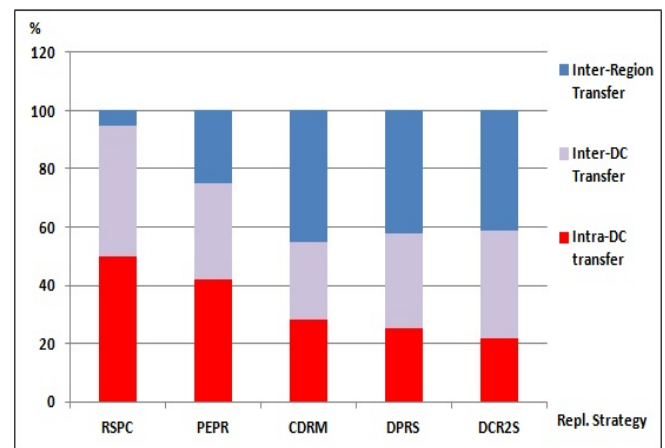
Figure 4 Average NB resource consumption
