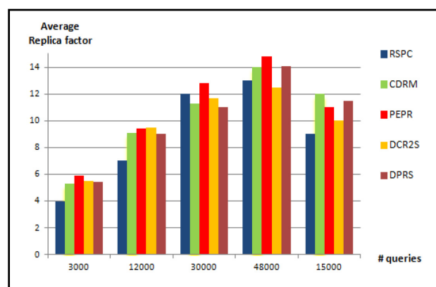
Figure 2 Average replica factor
