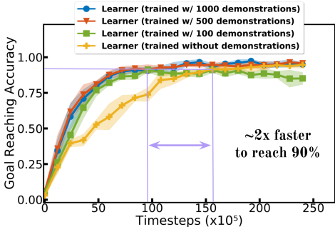
Fig. 4: Demonstrations double the learner’s training speed.
