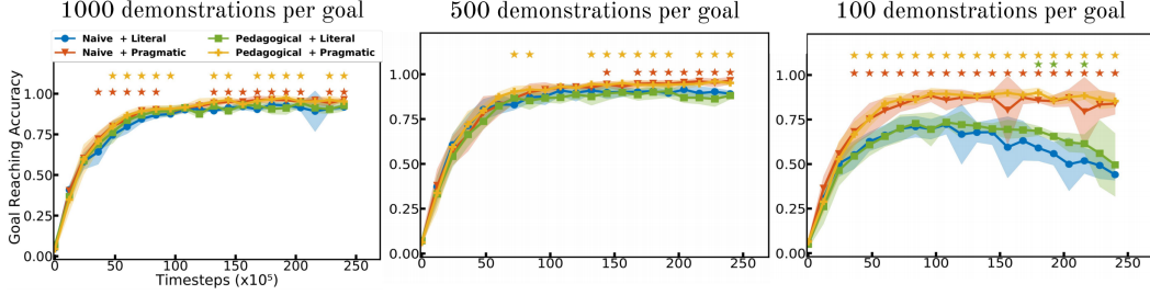
Fig. 3: Global learner performance in the FBS environment (Goal Reaching Accuracy, GRA) with different numbers of demonstrations per goal. Table 1 shows that the drop in GRA under the few demonstrations regime (right) is mainly due to incorrect goal inference in the literal learner or with the naive teacher. Stars indicate significance (tested against naive+literal).
