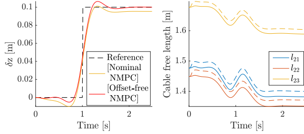
Fig. 8: On the left, step responses of the nominal NMPC and offset-free NMPC for an inaccurate value of the CDPR mass. On the right, corresponding cable free lengths \mathbf{l}_2 (solid lines) versus the estimated lengths \hat{\mathbf{l}}_2^* (dashed lines).
