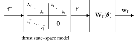
(a) Model with thrust dynamics.
