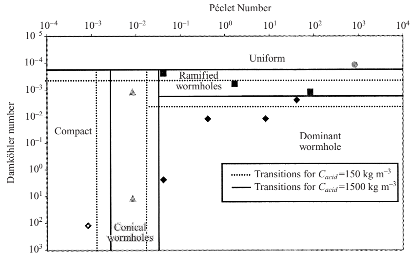
FIGURE 19. Concentration effect on the regime diagram; L = 10 cm.
