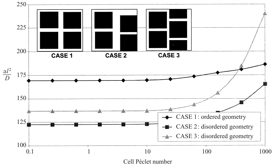
FIGURE 28. Comparison of the values of the transference coefficient, \alpha , for different geometries, \epsilon_\beta = 0.2 .
