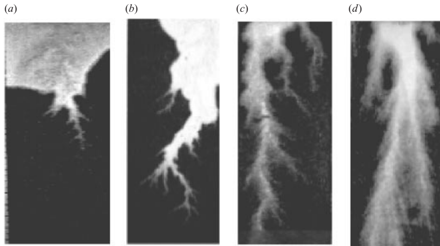
FIGURE 4. Example of experimental patterns of dissolution: (a) face dissolution, Q = 5 \text{ cm}^3 \text{ h}^{-1} , C_{NaCl} = 150 \text{ g l}^{-1} ; (b) conical wormhole, Q = 10 \text{ cm}^3 \text{ h}^{-1} , C_{NaCl} = 230 \text{ g l}^{-1} ; (c) dominant wormhole, Q = 50 \text{ cm}^3 \text{ h}^{-1} , C_{NaCl} = 150 \text{ g l}^{-1} ; (d) ramified wormhole, Q = 250 \text{ cm}^3 \text{ h}^{-1} , C_{NaCl} = 150 \text{ g l}^{-1} .
