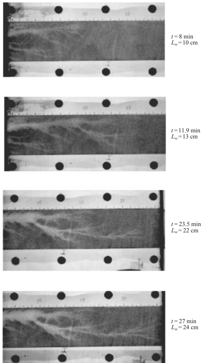
FIGURE 5. Dissolution history in the wormholing regime; C_{NaCl} = 150 \text{ g l}^{-1} , Q = 50 \text{ cm}^3 \text{ h}^{-1} .
