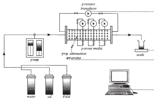
Fig. 3—Experimental setup.
