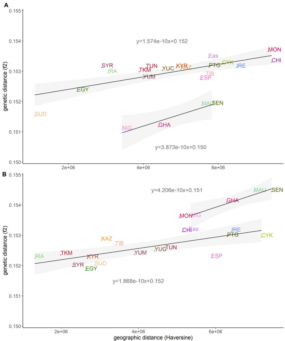
Fig. S5: Genetic distance ( f_2 , estimated using ADMIXTOOLS2) ( 123 , 124 ) verses geographical distance (estimated as haversine distance) from: A) donkeys from Ethiopia, and B) donkeys from Yemen. Two separate linear regressions were fitted for each dataset: one for subpopulations from Western Africa only, and another for all other subpopulations. F_2 statistics were estimated for all phased SNPs, but masking regions that were attributed to wild ancestry as estimated using PCAdmix ( n=11,577,531 variants, TI/TV=2.18 ).
