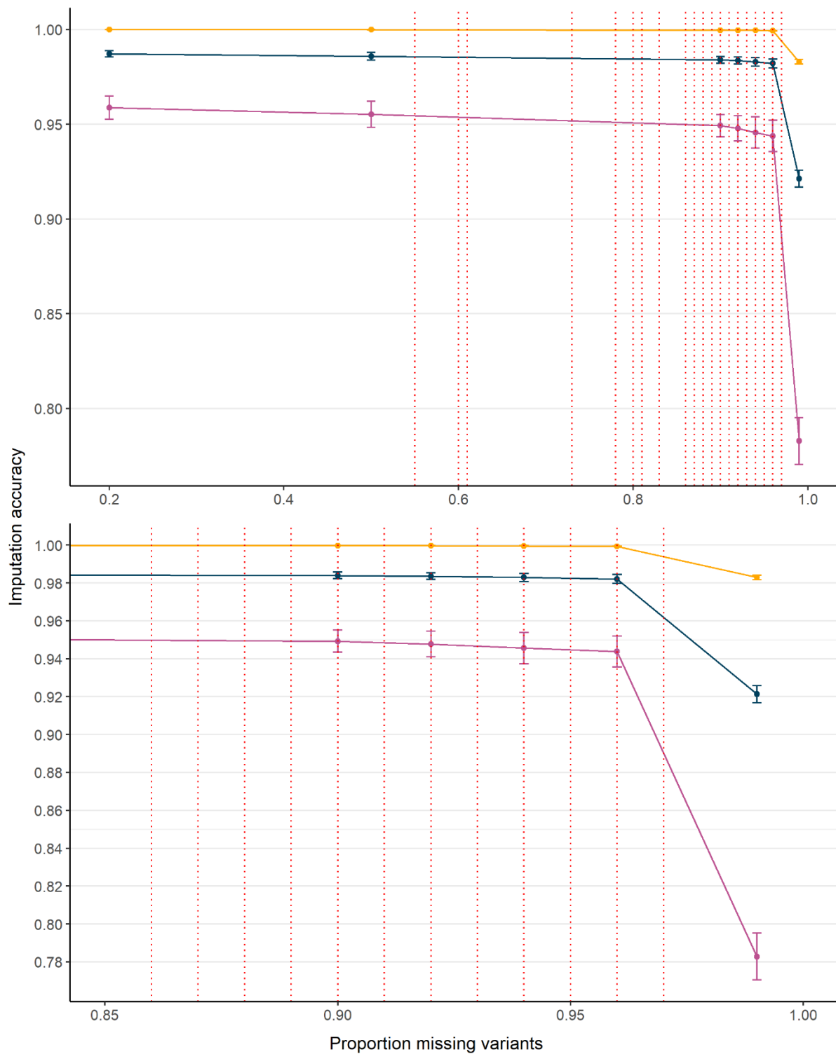
Fig. S8: The imputation accuracy versus the proportion of missing variants before imputation as estimated by downscaling modern donkey variants ( n=10 individuals). Accuracy of all variants (blue), homozygotes only (yellow) and heterozygotes only (purple) and plotted separately. The same imputation pipeline was used as that to impute the ancient donkey genomes. The proportion of missing variants for each ancient sample ( n=31 ) are shown as red dotted lines.
