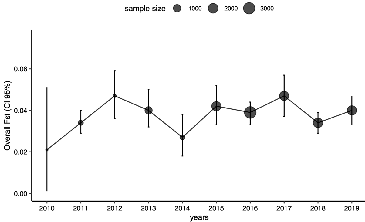
Figure 1. Genetic differentiation (multilocus Fst) amongst patches over 10 years. Dots and bars around the dots correspond respectively to global Fst estimates measured amongst patches and their associated 95% confidence intervals. Dot size is proportional to the sample size used to estimate Fst.
