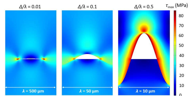
Figure 2: Spatial variation of the maximal shear stress \tau_{max} around the BII for BIC = 50% and three values of the implant roughness ( \Delta/\lambda = 0.01, 0.1 , and 0.5 ).
