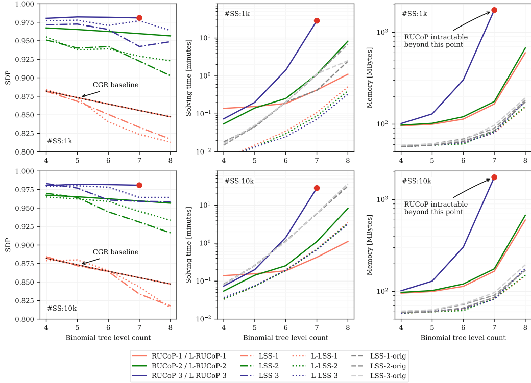
Fig. 6. SDP, solving time, and memory for binomial networks with varying complexity.
