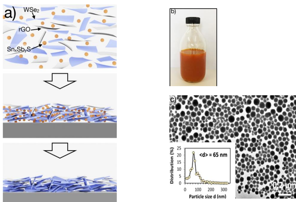
Figure 1: a) Schematic of the co-self-assembly process. b) Photograph of ( \text{Sn}_{0.5}\text{Sb}_{0.5}\text{S}_{1.5} ) template colloidal dispersion in DMF c) TEM image showing monodisperse spherical ( \text{Sn}_{0.5}\text{Sb}_{0.5}\text{S}_{1.5} ) colloids.
