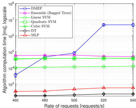
Figure 2: Comparison of the considered supervised learning approaches against the optimal solution (DMEP) in terms of computation time ( D_j^{max} \in [10, 100] ms).
