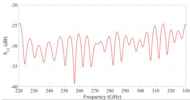
Fig. 2. Simulated magnitude of the reflection coefficient at the input port.
