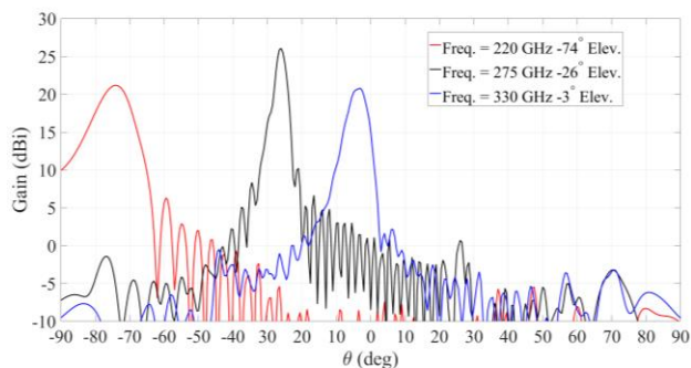
Fig. 3. Simulated radiation patterns in E-plane (xz-plane in Fig. 1). The pointing directions for each beam are provided in the legend.
