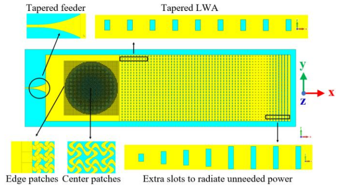
Fig. 1. Top view of the full antenna system.
