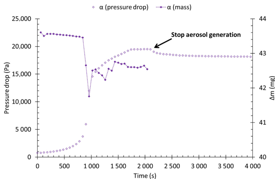
Figure 10. Pressure drop and mass evolution, before and after the aerosol stop, as a function of time, for filter \alpha (at 6 cm/s).
