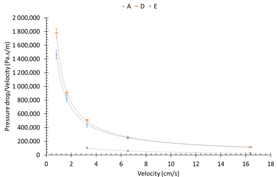
Figure 8. Aerodynamic resistance, at the saturation, as a function of filtration velocity.
