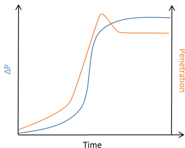
Figure 1. Pressure drop evolution and penetration (for particles <math>< 10 \mu\text{m}</math>) as a function of time.
