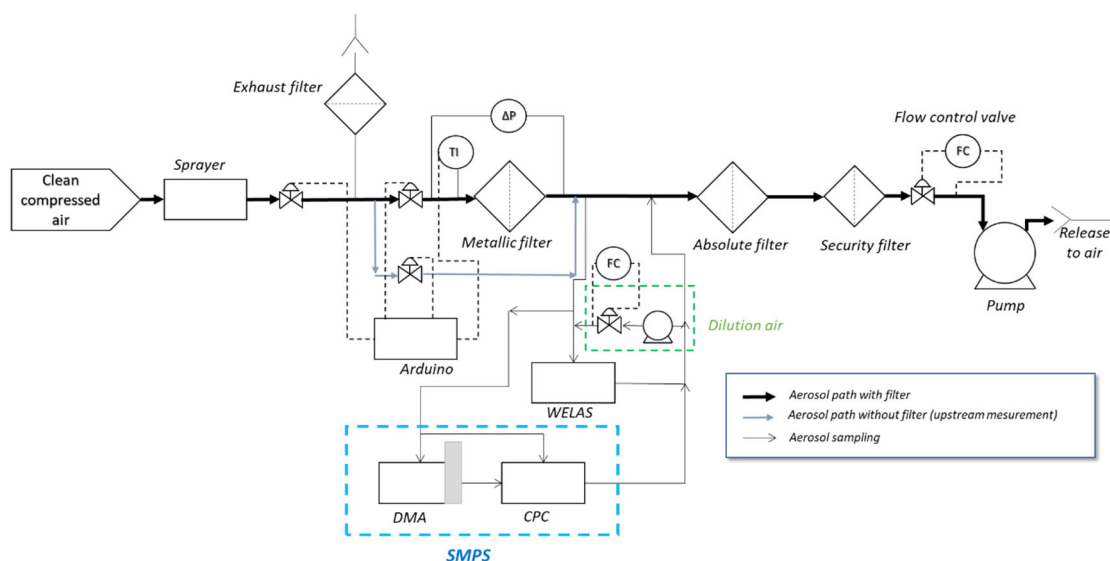
Figure 2. Experimental set-up.
