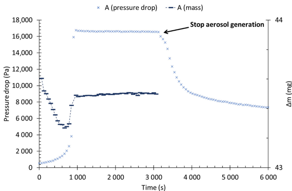
Figure 6. Pressure drop and collected mass, before and after the liquid aerosol stop, as a function of time at a filtration velocity of 6 cm/s (Filter A).
