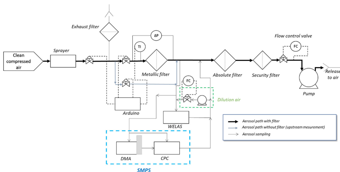
Figure 2. Experimental set-up.
