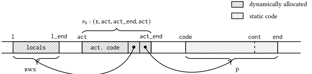
Fig. 11. Heap-based calling convention, with a the first instruction in the call macro
