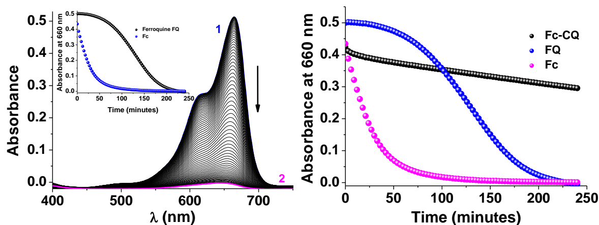
Figure 12. (left) Visible absorption spectral variation centred on MB along the Fenton reaction catalyzed by FQ in aqueous solution. (inset: variation of the absorbance at 660 nm as a function of time for FQ compared to Fc ). (right) variation of the absorbance at 660 nm (absorption of MB ) as a function of time for FQ compared to Fc and an equimolar mixture of Fc and CQ . Solvent: water at pH 3; T = 37.0\text{ }^{\circ}\text{C} ; l = 0.2\text{ cm} . [\text{MB}]_0 = 3 \times 10^{-5}\text{ M} ; [\text{Fc}]_0 = [\text{FQ}]_0 = [\text{CQ}]_0 = 9.5 \times 10^{-5}\text{ M} ; [\text{H}_2\text{O}_2]_0 = 3.26 \times 10^{-2}\text{ M} .
