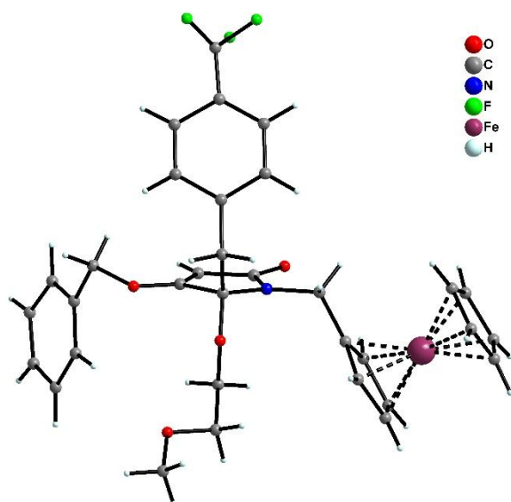
Figure 5. Single-crystal X-ray diffraction analysis of lactam 33
