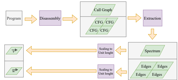
Fig. 2: PSS preprocessing.
