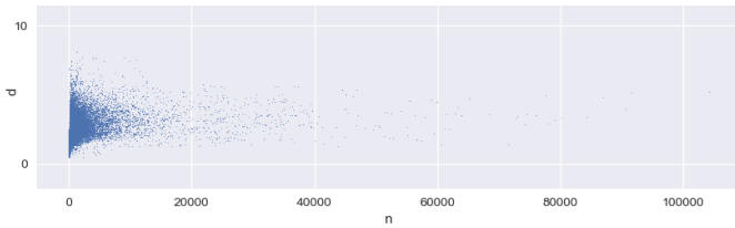
Fig. 11: A restricted plot of call graphs average degree against their number of nodes.
