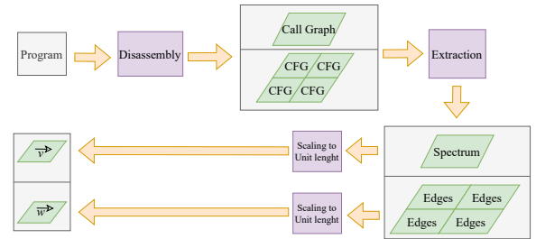
Fig. 2: PSS preprocessing.
