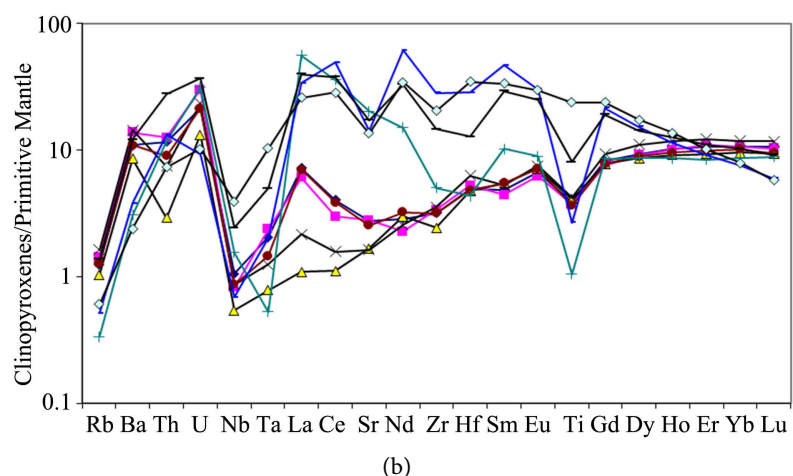
Figure 4. Clinopyroxene REE (a) and multi-element abundance (b) patterns normalised to the estimated primitive mantle values of Nyos peridotites. Normalization values after [32].
