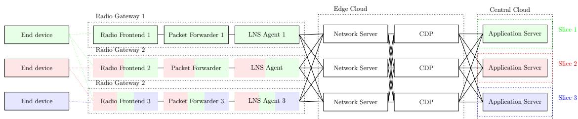
Figure 2.4: Gateway sharing a mutualized LNS infrastructure
