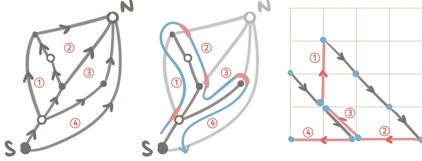
FIGURE 10. A bipartite plane bipolar orientation (left), and its rightmost incoming tree (middle), excluding the vertex N . The corresponding even tandem walk (right) is obtained by revolving around the tree in clockwise order: when first seeing an edge, it yields a SE step, and when first entering a face of type (i, j) , it yields a face-step (-i, j) .
