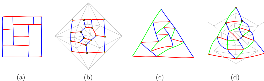
FIGURE 14. (a) a free bicolored contact-systems (corresponding to a plane bipolar orientation), (b) a rigid bicolored contact-systems (dual to a transversal structure), (c) a free tricolored contact-systems (corresponding to a polyhedral orientation), (d) and a rigid tricolored contact-system (dual to a Schnyder labeling).
