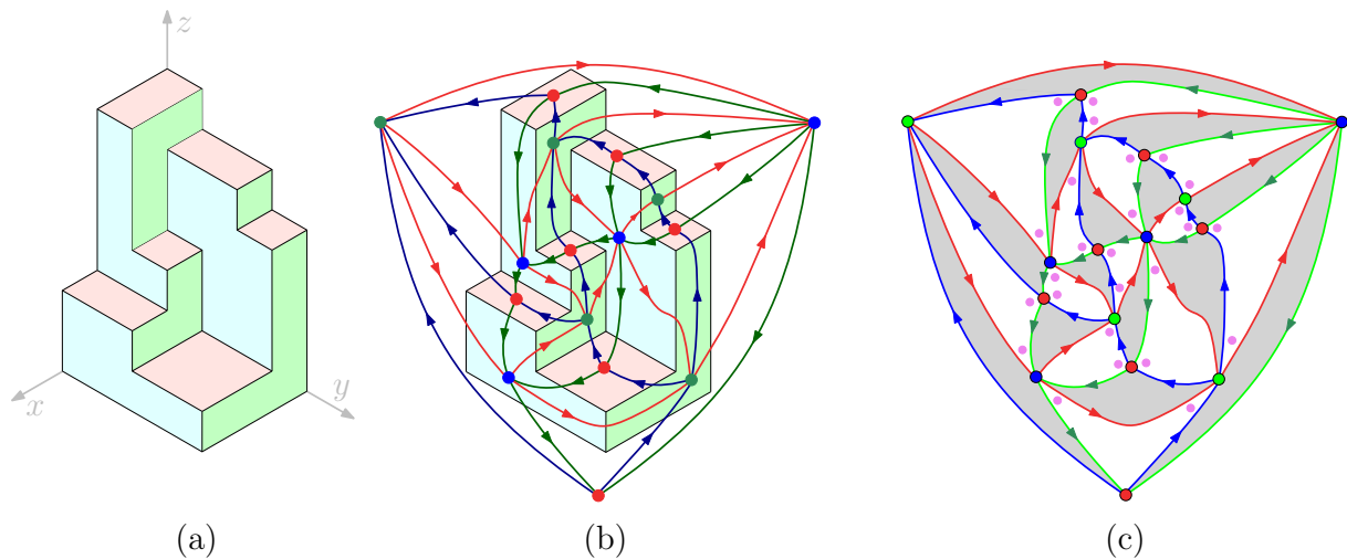
Figure 2: From a corner polyhedron to an Eulerian triangulation endowed with a polyhedral orientation (extremal corners are indicated in violet, there are two such corners at each inner vertex and at each light inner face).
