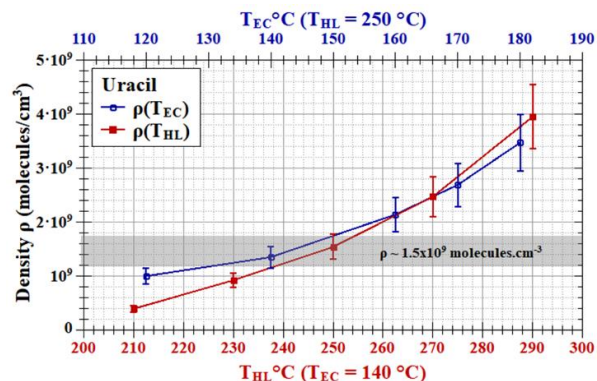
Figure 6: Evolution of uracil density as a function of oven temperatures T_{\text{EC}} (blue open circle) and T_{\text{HL}} (red full square). The uncertainty is estimated to be around 19% and takes into account both systematic errors on the estimation of the length l ( \Delta l/l \sim 9\% ) and the temperature T ( \Delta T/T \sim 4\% ) and statistical errors on the measure of the mass flux \Phi by the quartz crystal microbalance ( \Delta\Phi/\Phi < 5\% where \Delta\Phi is the standard deviation).
