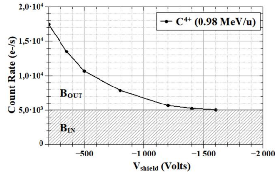
Figure 8: Count Rate of background signal (i.e. electron emission from residual gas) as a function of the potential applied to V_{\text{shield}} ( = V_0 = V_1 ) for the projectile C^{4+} ion beam at 0.98-MeV/u kinetic energy. The measurement is performed for the VMI extraction V_{\text{ext}} = 1000 V.
