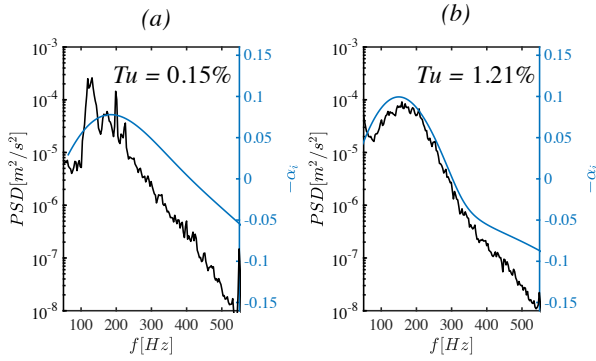
Figure 5. Comparison between the amplified frequencies predicted by LST to the experimental spectra for (a) Natural case ( x = 0.400c ); (b) Tu = 1.21\% ( \Lambda_u = 8.7mm , x = 0.425c ); NB: Two different y -axes for \alpha_i and the power from the PSD, therefore direct comparisons between the two are not be made.
