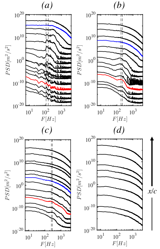
Figure 4. Chordwise evolution of the PSD. Frequency bands correspond to the vertical dashed lines which indicate the most amplified frequency band used in the stability analysis in the following section. Red and blue curves denote x_S and x_R , respectively. NB: Spectra are separated by an order of magnitude for clarity. a) Tu = 0.15\% . Frequency band: [110-150 Hz]; b) Tu = 1.21\% . Frequency band: [180-220 Hz]; c) Tu = 2.97\% . Frequency band: [255-295 Hz]; d) Tu = 6.28\% ;
