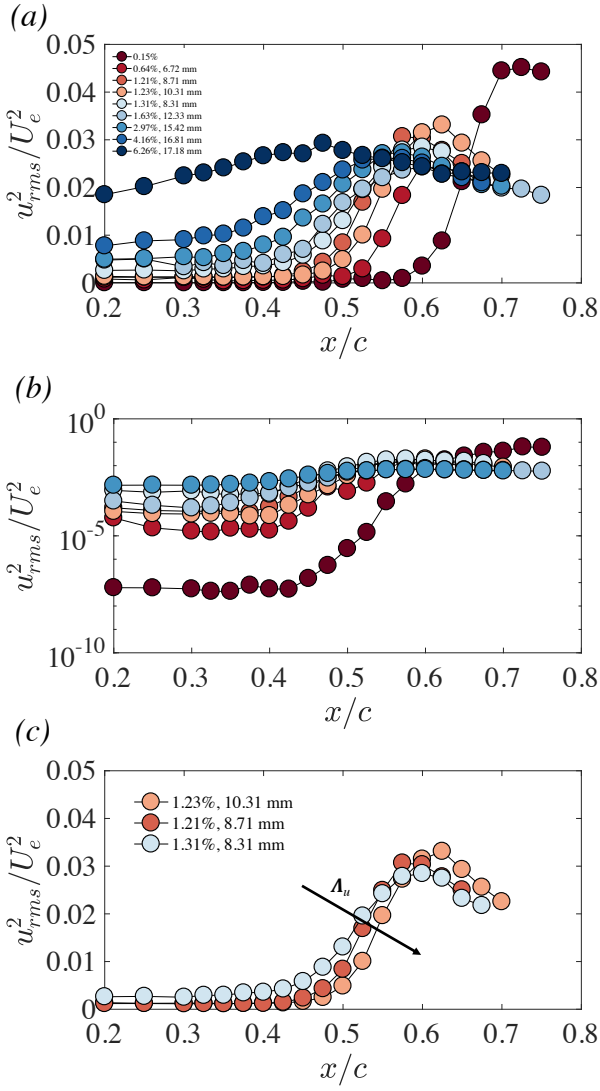
Figure 3. The disturbance energy growth for a) integrated over the entire energy spectrum and b) integrated over the frequency range of the most amplified wave packet and c) configurations with are latively fixed Tu and varying \Lambda_u .
