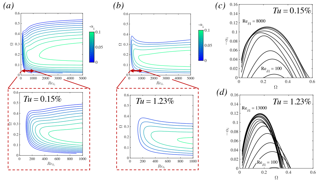
Figure 7. Contours of LST predicted spatial growth rates ( \alpha_i ) as a function of the dimensionless frequency \Omega and Reynolds number ( Re_{\delta_1} ) for the natural case for a mean velocity profile at x = 0.400c (a) and an elevated freestream turbulence case for a mean velocity profile at x = 0.425c (b). The dependence of \alpha_i on Re_{\delta_1} is presented in (c) and (d) for the natural and exited case, respectively. In both configurations the initial value of Re_{\delta_1} = 100 and continues up until the maximum \alpha_i converges within 2%.
