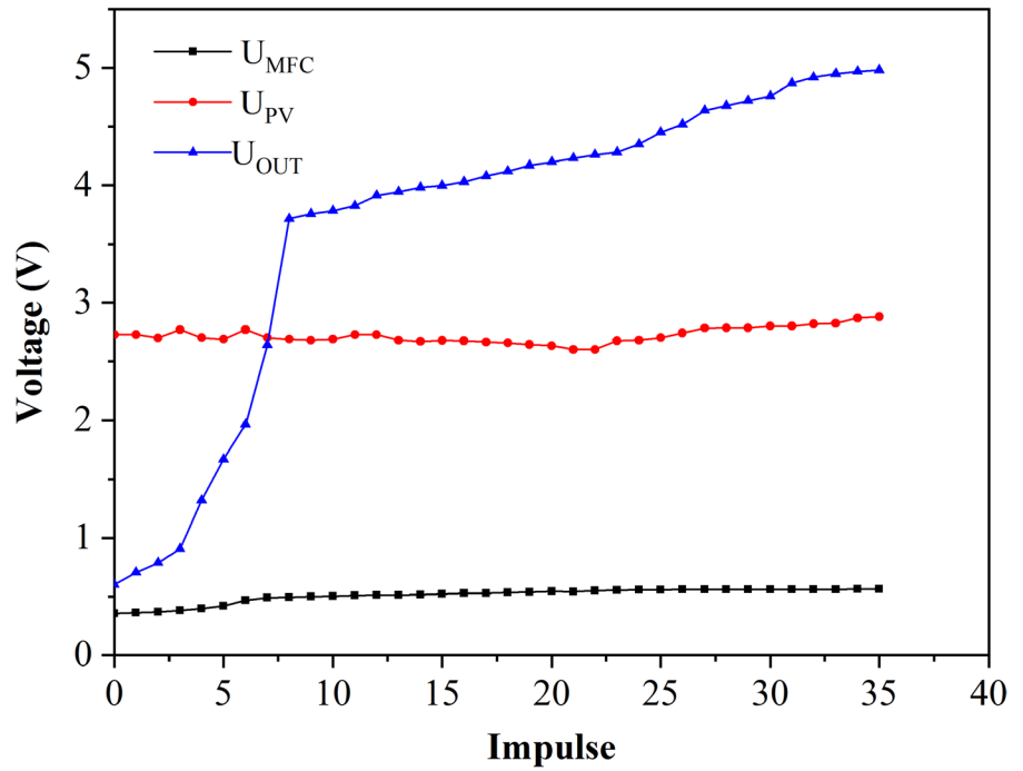
Fig. 6 Evolution of output amplified voltage of the MFC using solar panel polarization and DC/DC boost converter
