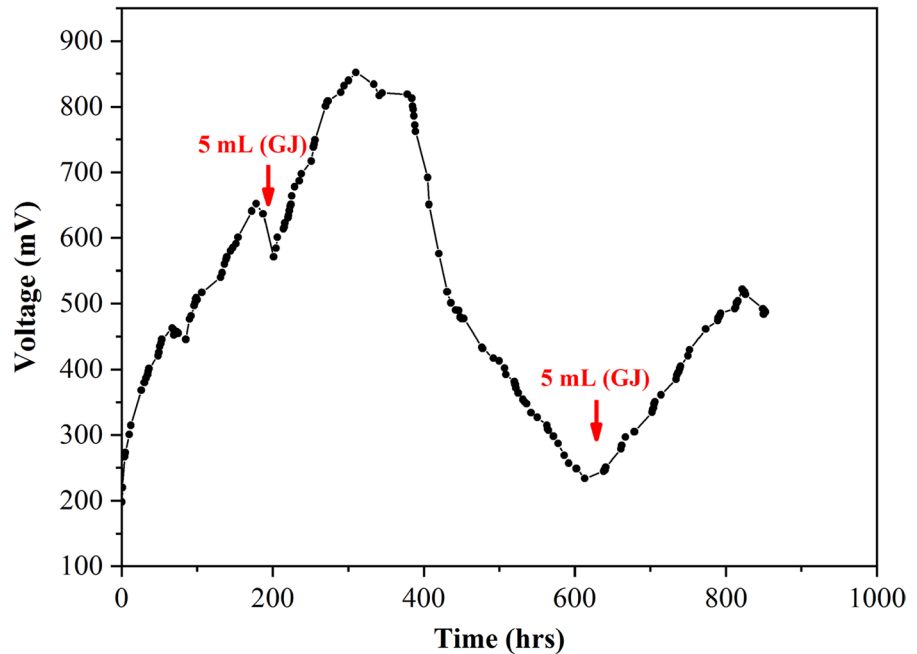
Fig. 1 Evolution of the open circuit voltage of the sheep manure microbial fuel cell (MFC) during 870 h
