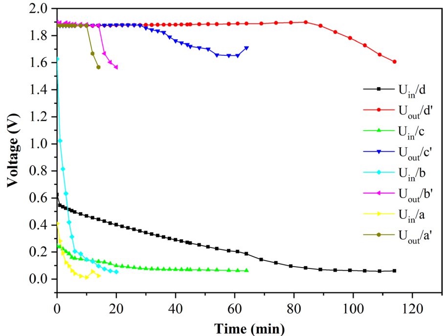
Fig. 4 Evolution of input and amplified voltages using different configurations: (a–a') single stack of MFC; (b–b') series association of MFCs; (c–c') parallel association of MFCs; (d–d') parallel association of MFCs with polarization voltage
