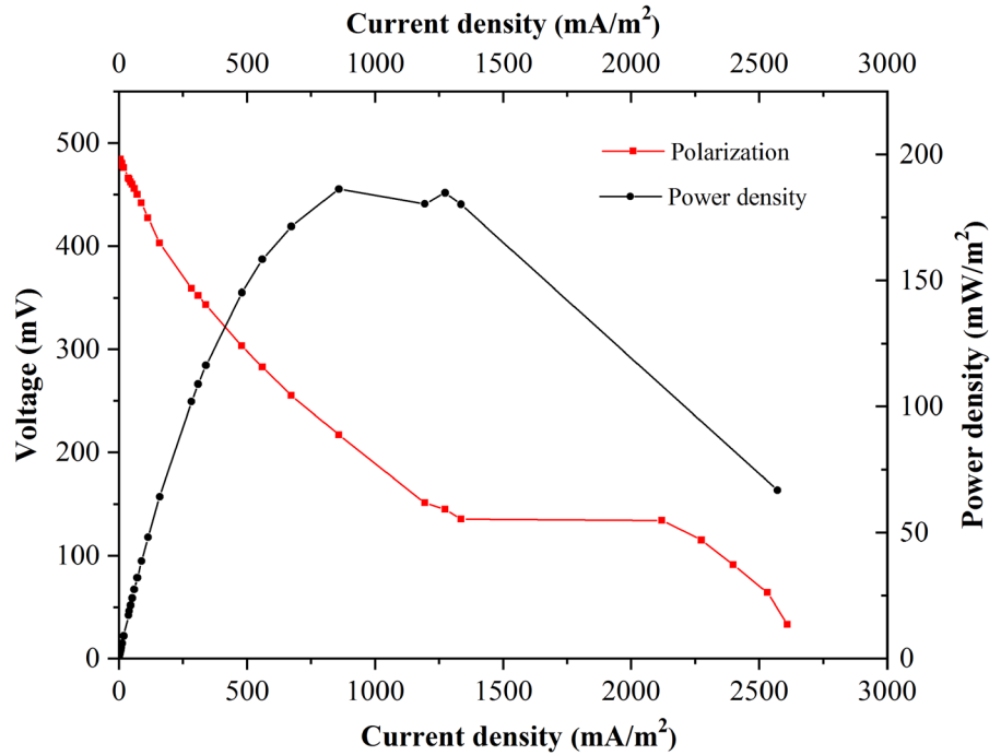
Fig. 2 Polarization and power density curves during the MFC operation (obtained after discharging to different external electrical resistances)
