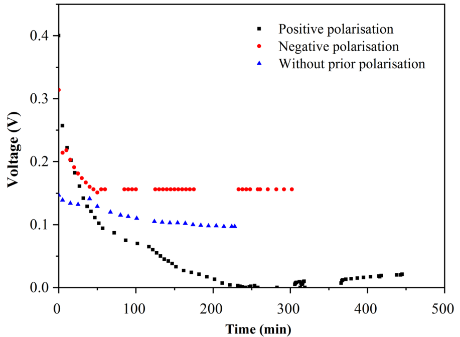
Fig. 3 Evolution of the MFC discharged to external electric resistance 1000 \Omega upon positive and negative polarizations
