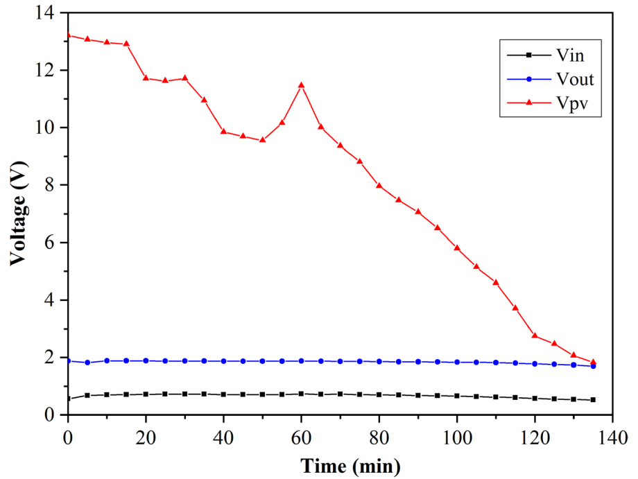
Fig. 5 Evolution of output amplified voltage of the MFC using an amplifier polarized with a solar panel
