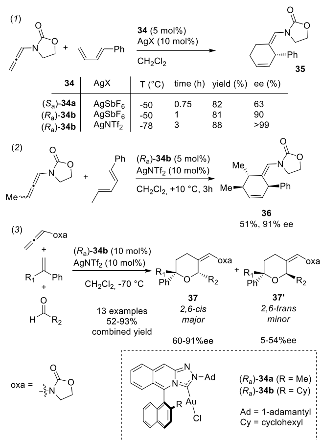
Figure 14. Enantioselective [4+2] cycloaddition of allenamides with dienes and [2+2+2]-cycloaddition of allenamide, alkenes and aldehydes catalyzed by complexes 34 .
