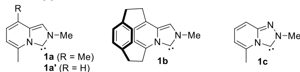
Figure 2. Control over the cycloaddition of eneallene 2 through electronic tuning of N-heterobicyclic carbene ligands 1a-c .
