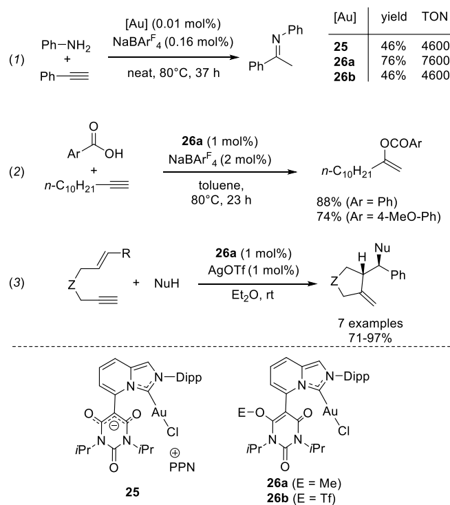
Figure 10. Intermolecular hydroamination and hydrocarboxylation of alkynes and domino hydroamination and hydrocarboxylation of alkynes and domino
