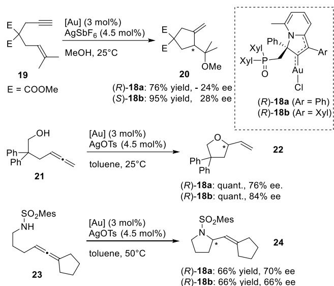
Figure 8. Asymmetric methoxycyclization, intramolecular hydroalkylation and hydroamination catalyzed by gold(I) catalysts 18a-b . Xyl = 3,5-xylyl.
