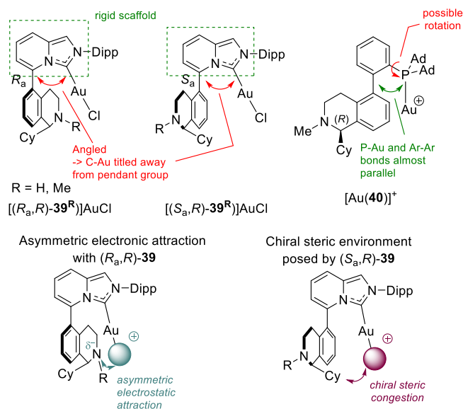
Figure 16. Chiral bifunctional ImPy-gold(I) complexes AuCl( 39 ), comparison to bifunctional phosphine 40 , and proposed modes of inducing chirality depending on the chiral axis configuration.
