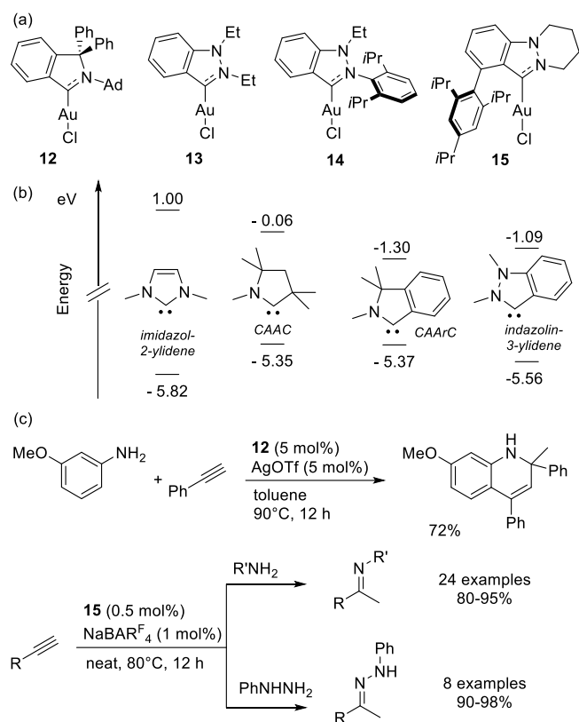
Figure 6. (a) Reported Au(I) complexes with CAACr and indazolin-3-ylidene ligands. (b) Calculated energy for the HOMO and LUMO of imidazol-2-ylidene, CAAC, CAACr, and indazolin-3-ylidene for comparison (B3LYP/def2-TZVPP level of theory). Values taken from ref [21] (c) Three component synthesis of 1,2-dihydroquinoline catalyzed by 12 . Hydroamination and hydrohydrazination of acetylenes with 15 .
