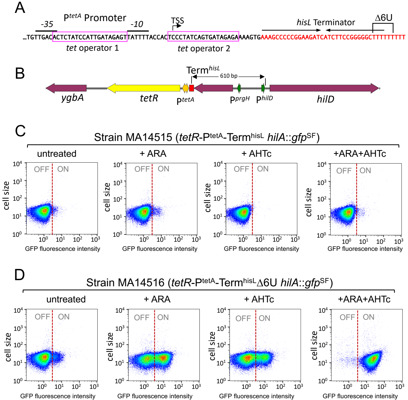
Fig. S6. Rho-independent transcription terminator abolishes the effects of NusG depletion on SPI-1 bistability. (A) Sequence of the P tetA -Term hisL fusion in strains MA14515 (wt terminator) and MA14516 (Δ6U mutant), respectively. (B) Schematic diagram showing Term hisL position relative to P tetA and P hilD (secondary hilD promoters not shown). (C) and (D) Representative flow cytometry analysis of cells from strains MA14515 (C) and MA14516 (D). See legend in next page for details.
