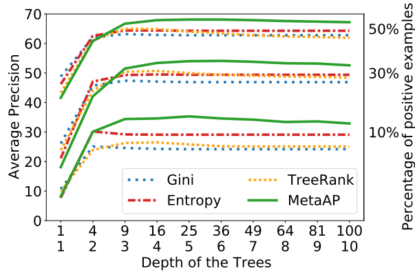
Figure 5: Mean AP as a function of the depth on the public datasets with a proportion of positives of at most 10%, 30% and 50%. The 1st line ( resp. 2nd) of the x-axis represents the depth of the Gini and Entropy -based DTs ( resp. TreeRank and MetaAP ).
