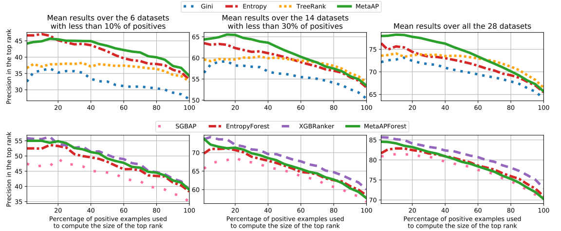
Figure 6: Precision@k according to the percentage of positives. (Top) DT methods. (Bottom) RF and Gradient Tree Boosting methods.
