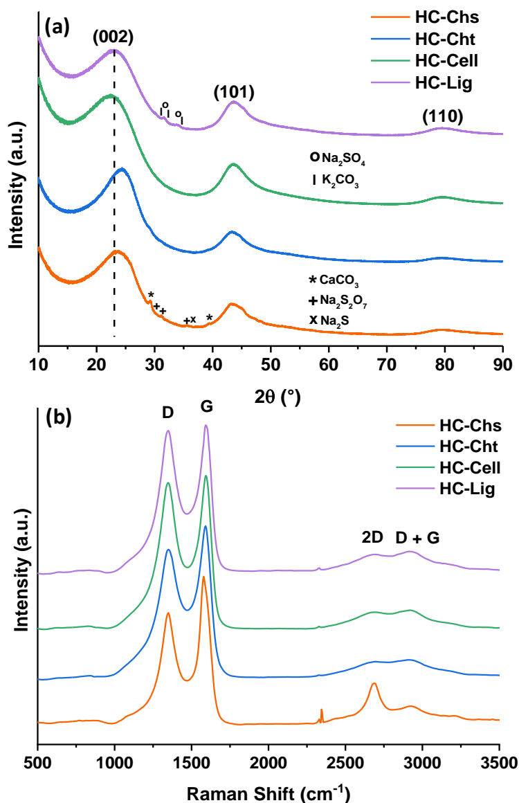
Figure 1: Cu ( \text{K}\alpha_{1,2} ) XRD-diffractograms (a); impurities are partially indicated (only strongest reflexions) and averaged Raman spectra (b) of hard carbon materials: HC-Chs, HC-Cht, HC-Cell and HC-Lig.
