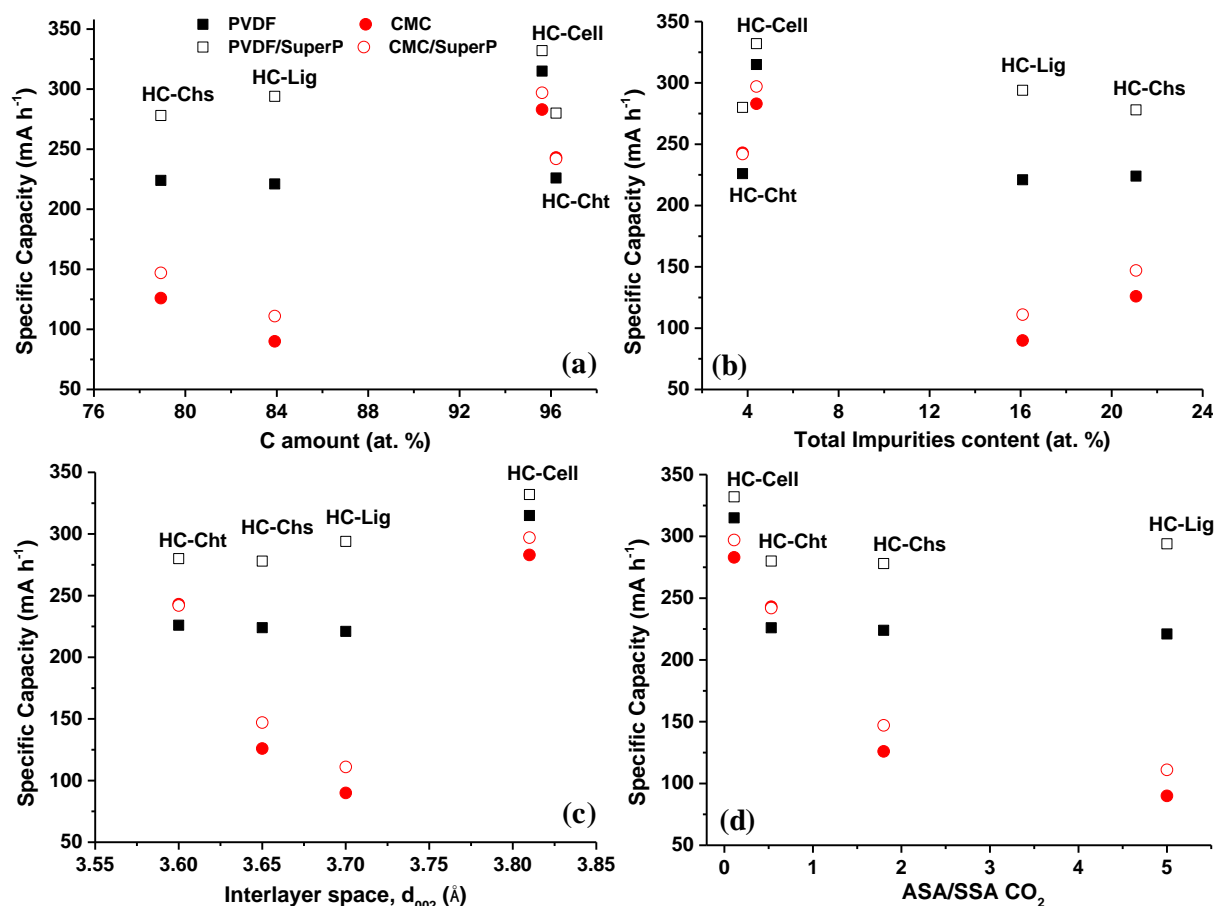
Figure 10: Correlation between the specific capacity and (a) the carbon amount (b) the level of impurities (including inorganic impurities, and oxygen- and other heteroatom-containing impurities detected by XPS), c) the interlayer spacing, d_{002} , and (d) the ratio of ASA to SSA CO 2 , for all four hard carbons formulated with PVDF and CMC binders without and with SuperP and tested in 1M NaPF 6 in EC:DEC.
