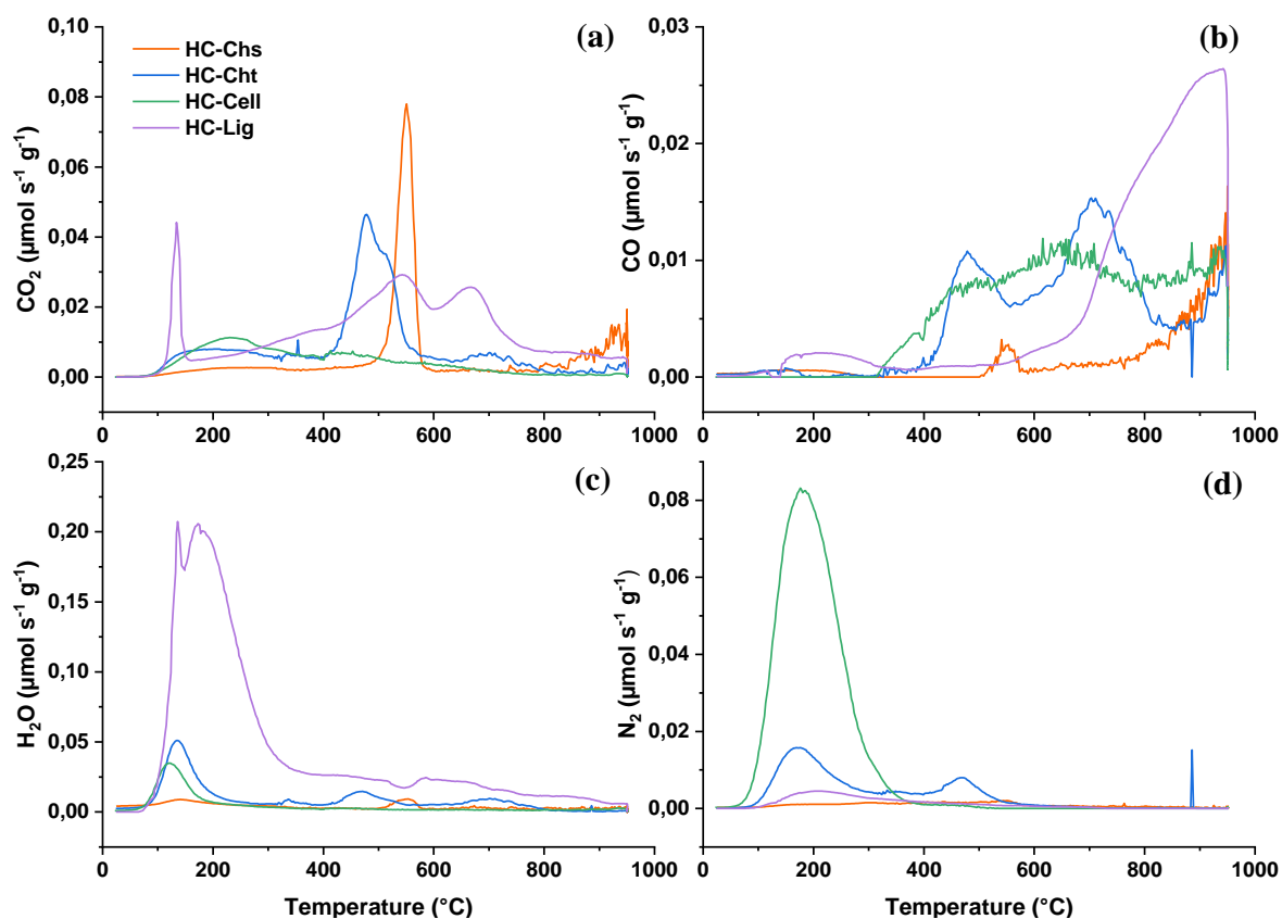
Figure 4: Gas desorption profiles of (a) CO 2 , (b) CO, (c) H 2 O and (d) N 2 obtained by TPD-MS for HC-Chs, HC-Cht, HC-Cell and HC-Lig hard carbons.
