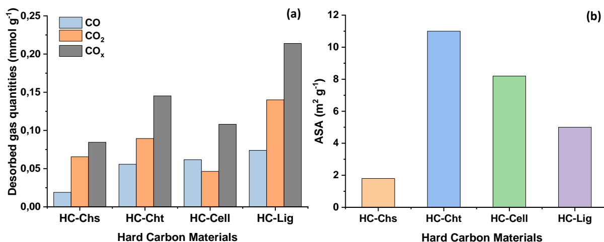
Figure 5: (a) Desorbed amounts of CO, CO 2 and CO x (CO + CO 2 ) gases released by thermal decomposition during the TPD-MS experiment and (b) the active surface area (ASA) of hard carbon materials.
