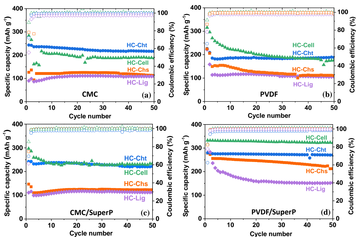
Figure 6: Specific charge capacity (full symbols) and Coulombic efficiency (empty symbols) of the Na-ion half-cells tested with electrodes based on four different HCs formulated with (a) CMC, (b) PVDF (c) CMC /Super P and (d) PVDF/SuperP binders in 1 M NaPF 6 in EC:DEC electrolyte. The first two cycles were performed at a rate of C/10. The rest of the cycling proceeded at a rate of C/5.
