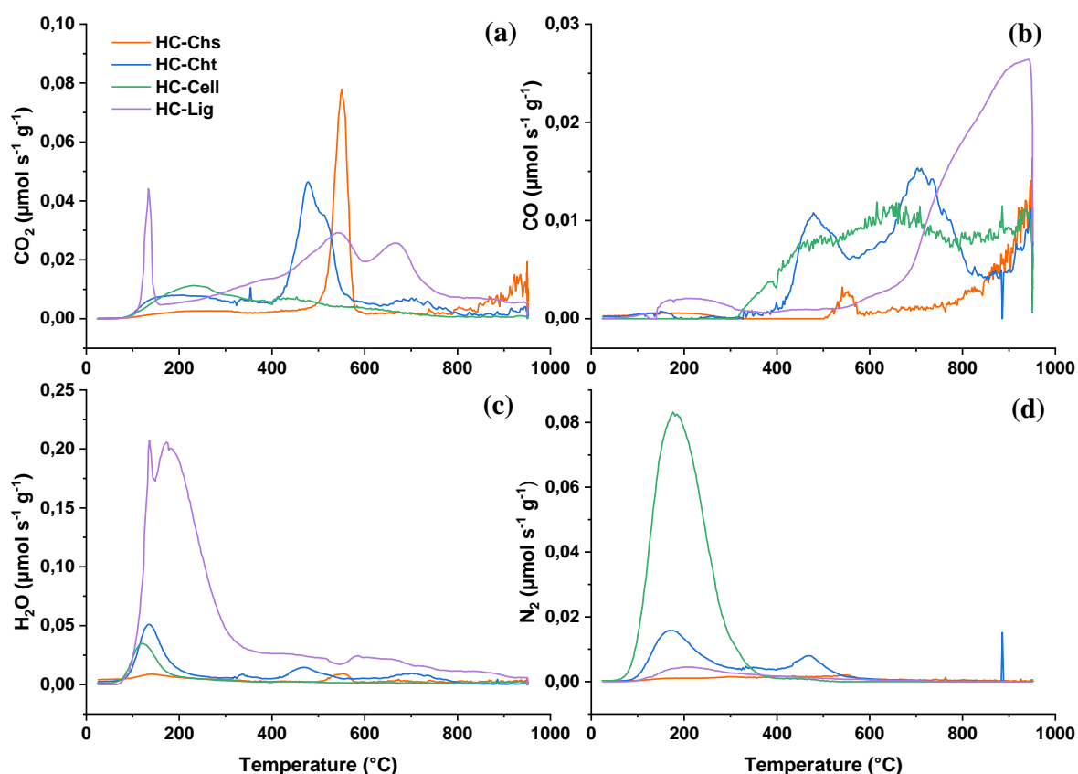
Figure 4: Gas desorption profiles of (a) \text{CO}_2 , (b) \text{CO} , (c) \text{H}_2\text{O} and (d) \text{N}_2 obtained by TPD-MS for HC-Chs, HC-Cht, HC-Cell and HC-Lig hard carbons.
