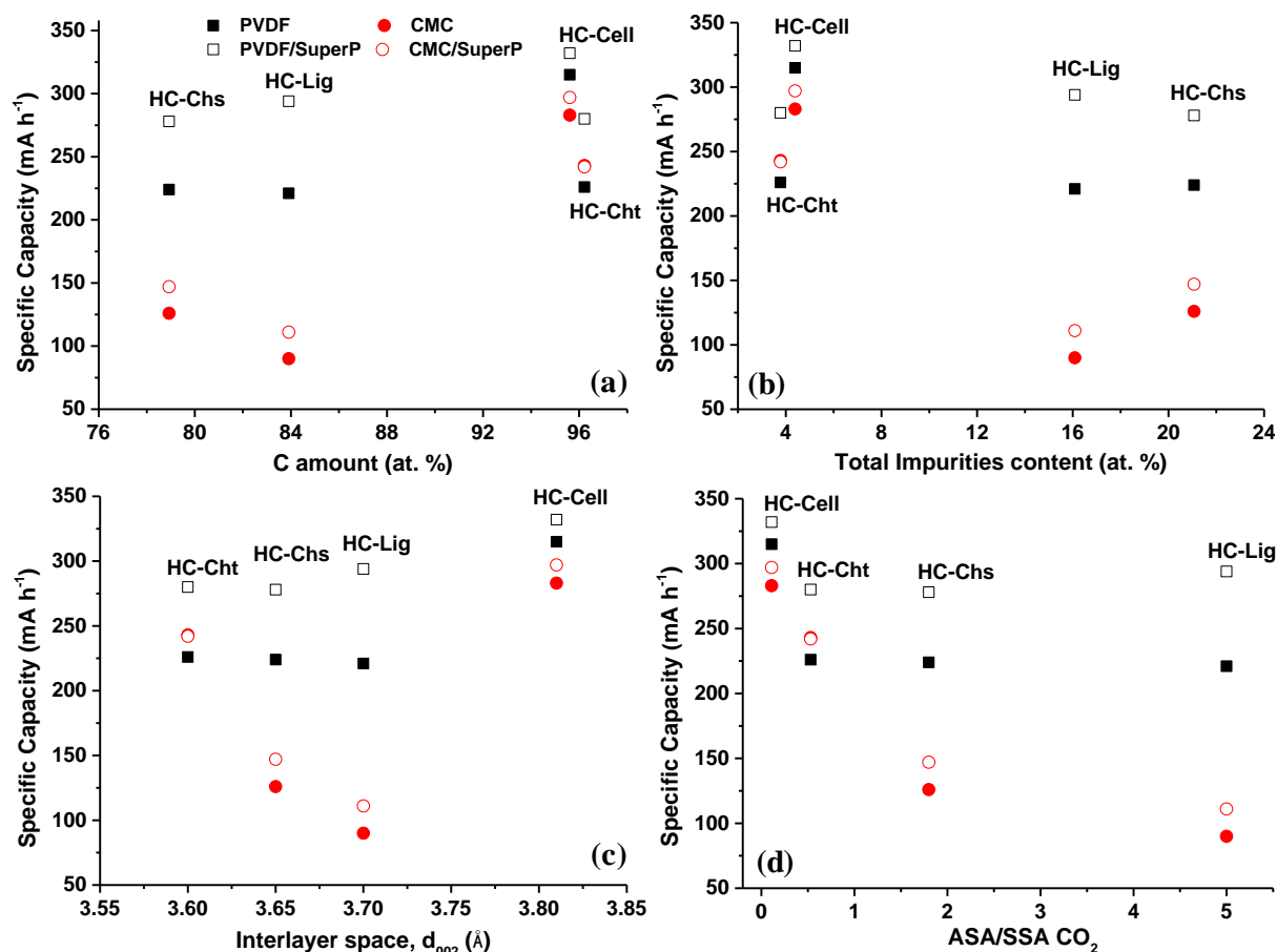
Figure 10: Correlation between the specific capacity and (a) the carbon amount ((b) the level of impurities (including inorganic impurities, oxygen- and other heteroatom-containing impurities), c) the interlayer spacing, d_{002} , and (d) the ratio of ASA to SSA CO 2 . for all four hard carbons formulated with PVDF and CMC binders without and with SuperP and tested in 1M NaPF 6 in EC:DEC.
