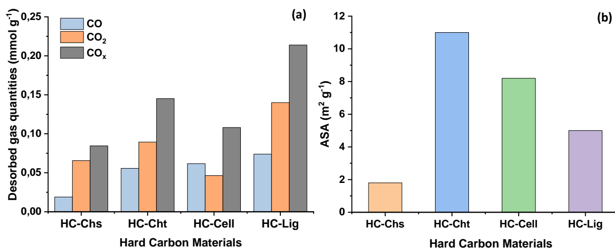
Figure 5: (a) Desorbed amounts of CO, \text{CO}_2 and \text{CO}_x ( \text{CO} + \text{CO}_2 ) gases released by thermal decomposition during the TPD-MS experiment and (b) the active surface area (ASA) of hard carbon materials.
