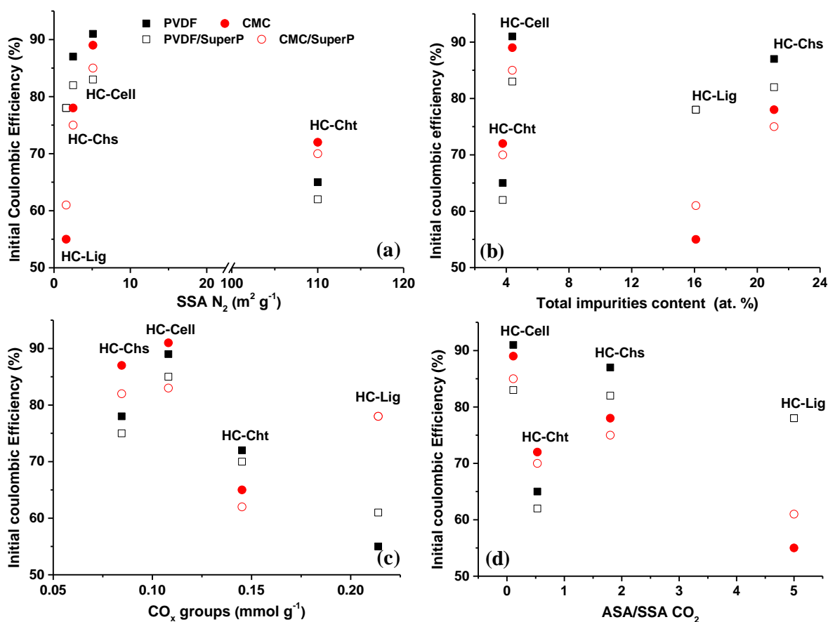
Figure 9: Correlation between the initial coulombic efficiency, iEC, and (a) the specific surface area, SSA N 2 , (b) the level of impurities (including inorganic impurities, oxygen- and other heteroatom-containing impurities), c) the oxygen-containing functional groups, CO x and (d) the ratio of ASA to SSA CO 2 for all four hard carbons formulated with PVDF and CMC binders without and with SuperP, and tested in 1M NaPF 6 in EC:DEC.
