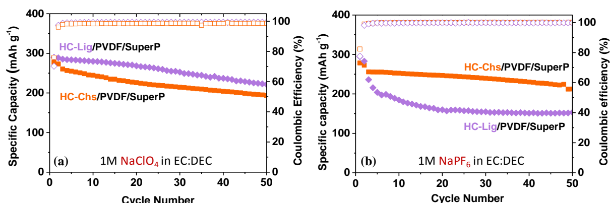
Figure 8: Specific capacity (full symbols) and Coulombic efficiency (empty symbols) of the Na-ion half-cells tested with electrodes based on HC-Lig and HC-Chs formulated with PVDF /SuperP, and (a) 1M NaClO 4 in EC:DEC and (b) in 1M NaPF 6 in EC:DEC.
