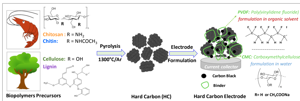
Scheme 1: Synthesis of hard carbon materials by pyrolysis of biopolymers and the electrode preparation.
