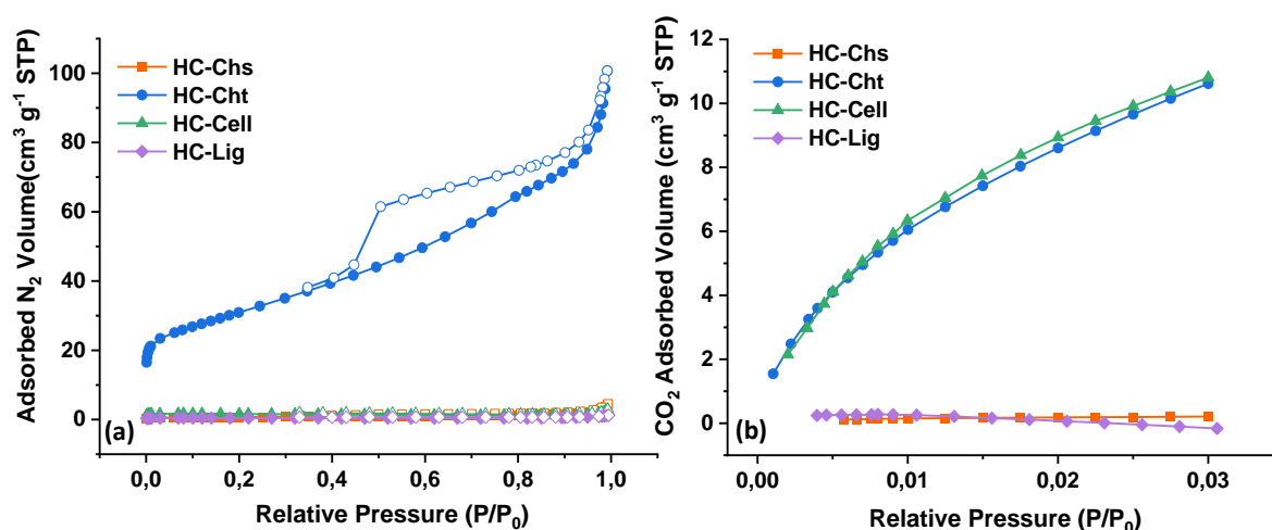
Figure 3: (a) Nitrogen adsorption/desorption isotherms measured at 77 K and (b) \text{CO}_2 adsorption isotherms measured at 273 K of HC materials: HC-Chs, HC-Cht, HC-Cell and HC-Lig.
