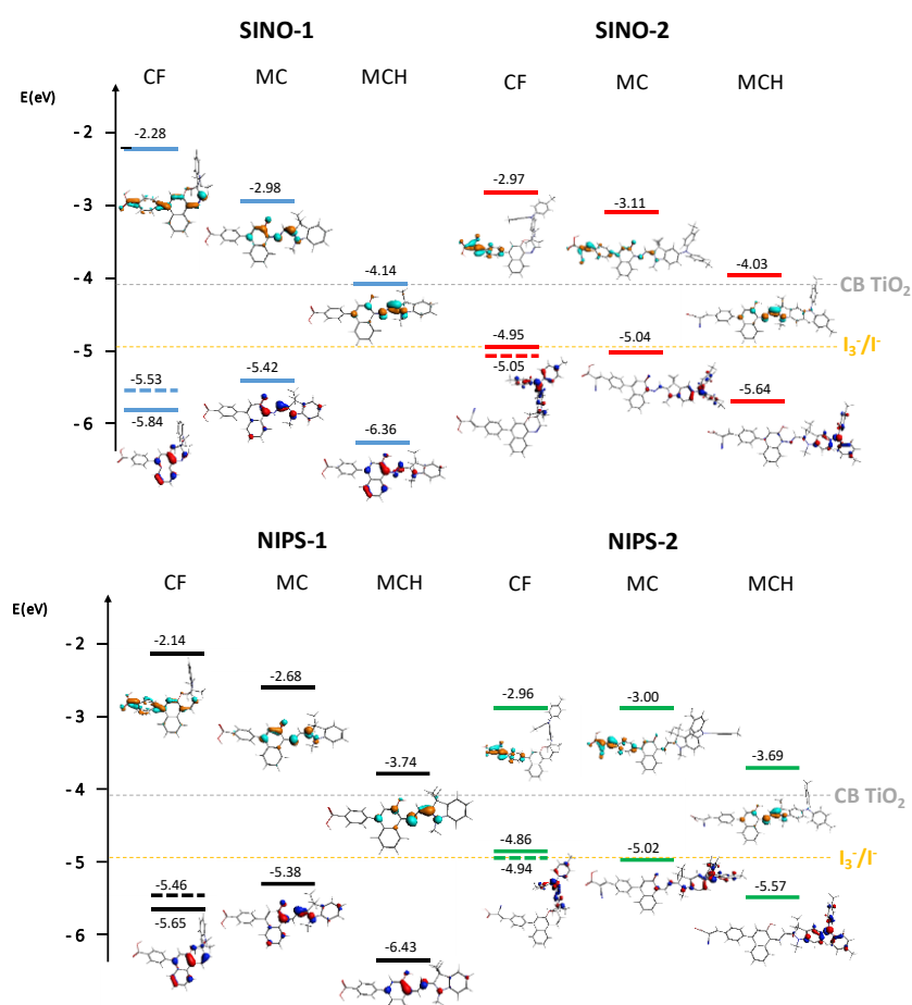
Figure 5. DFT-calculated energy levels (versus the vacuum level) of the frontier orbitals of the four new dyes and their spatial localizations in closed (CF), merocyanine (MC) and protonated merocyanine forms (MCH) (full lines). Experimental values of the CF obtained by CV are shown in dashed lines. The potential of the I 3 - /I - pair (ca. -4.95 eV) and the TiO 2 conduction band (ca. -4.10 eV) are shown in yellow and grey dashed lines respectively.
