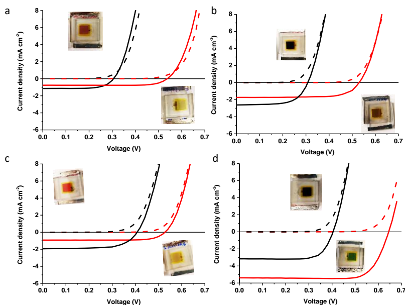
Figure 6. J-V curves of the 13 \mu m DSSCs using a) SINO-1 , b) SINO-2 , c) NIPS-1 , and d) NIPS-2 as sensitizers under standard irradiation conditions AM 1.5 G, 1000 W m -2 ; 25 °C (active area= 0.36 cm 2 ) using our homemade electrolyte (black) and Iodolyte (red) and the pictures of the respective devices in the absence of illumination.
