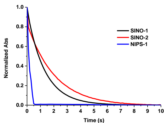
Figure 2. Normalized discoloration curves of SINO-1 , SINO-2 and NIPS-1 , example given in DMF in 2 \cdot 10^{-5} M solutions at 25 °C in the dark after irradiation 60 s with a 200-600 nm/200 W xenon lamp.
