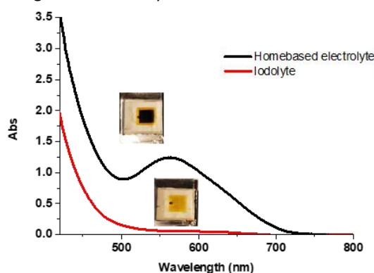
Figure 7. UV-Vis spectra and pictures of the respective devices of NIPS-2 -based DSSCs on 2 μm transparent TiO 2 electrodes using Iodolyte and our homebased electrolyte in the absence of illumination.
