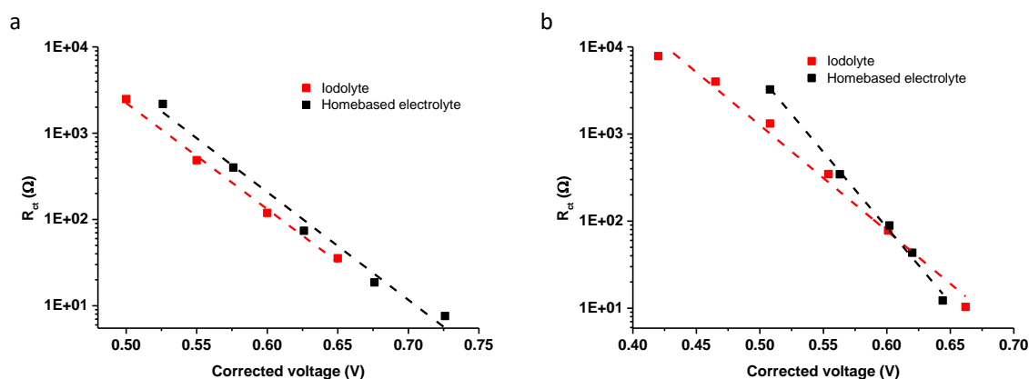
Figure 8. Charge transfer resistances comparisons at the same quasi-Fermi level of 13 \mu\text{m} DSSCs made of NIPS-2 and both electrolytes a) in the dark and b) under operating conditions.
