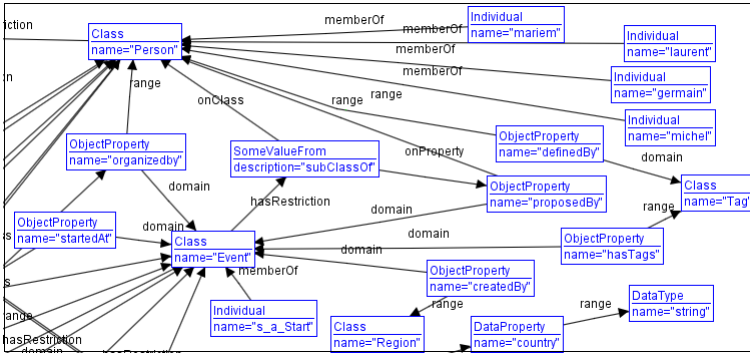
Fig. 10. EventCCAlps ontology after delete the "Employee" class.
