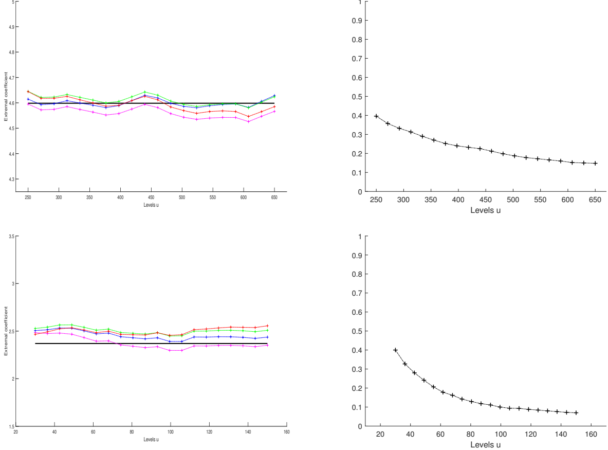
Figure 3: First row: \Lambda^2 \sim \text{Pa}(3/2) . Second row: \Lambda^2 \sim \text{Pa}(1/2) . Numerical illustrations related to extremal coefficients. Left panels: empirical estimation (in logarithmic scale) of \theta_S^{(*)} in (31) (black horizontal line), \theta_S^{(\star)}(u) in (32) (magenta crosses); \theta_S^{(k)}(u) in (33), for several large values of u and k = 2 (blue crosses), k = 1 (green crosses) k = 0 (red crosses), evaluated using 5000 i.i.d. simulations. Right panels: empirical estimated \mathbb{P}(\max_{s \in S} X^*(s) > u) , for the same levels u and the same simulations as in the corresponding left panels.
