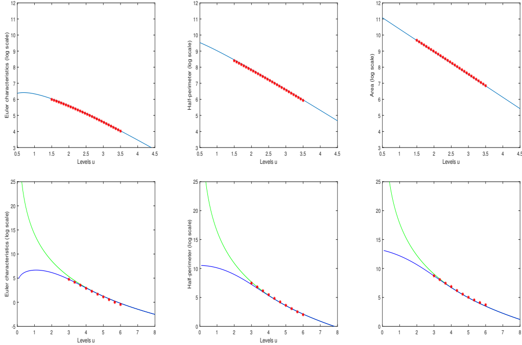
Figure 1: Illustration of expected LKCs. Shape variables are given as \Lambda^2 \sim \text{Exp}(1) (first row) and \Lambda^2 \sim \text{Pa}(4) (second row). Exact theoretical values of \mathbb{E}[\mathcal{L}_0(A(u, X, S))] (left panels), \mathbb{E}[\mathcal{L}_1(A(u, X, S))] (center panels) and \mathbb{E}[\mathcal{L}_2(A(u, X, S))] (right panels) are displayed in logarithmic scale with blue curves (see Table 1). Empirical means of estimated \mathcal{L}_k(A(u, X, S)) from 500 i.i.d. samples (red stars) are given for several values of u . In the second row, theoretical values of the asymptotic expected LKCs from Equation (26) in Proposition 2 are shown as green curves.
