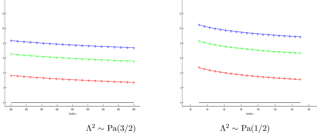
Figure 2: Averaged values (in logarithmic scale) of estimated \mathcal{L}_k(A(u, X^*, S)) based on 5000 i.i.d. sample simulations for k = 2 (blue circles), k = 1 (green circles) and k = 0 (red circles) for several large values of u . We also display the theoretical functions c_k^{scal}(\alpha, \lambda_2, S) u^{-1} with c_k^{scal} in (17) for k = 2 (blue curves), k = 1 (green curves) and k = 0 (red curves).
